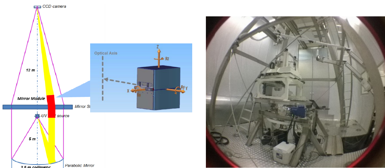
Figure 1. Schematic illustration of the alignment setup for the MM (left) and a picture of the actual optical bench (right).
