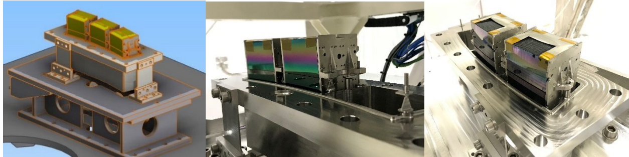
Figure 9. Demonstrator design (left) and build (centre, right) with two SPO MMs aligned and integrated on the mirror structure element.
