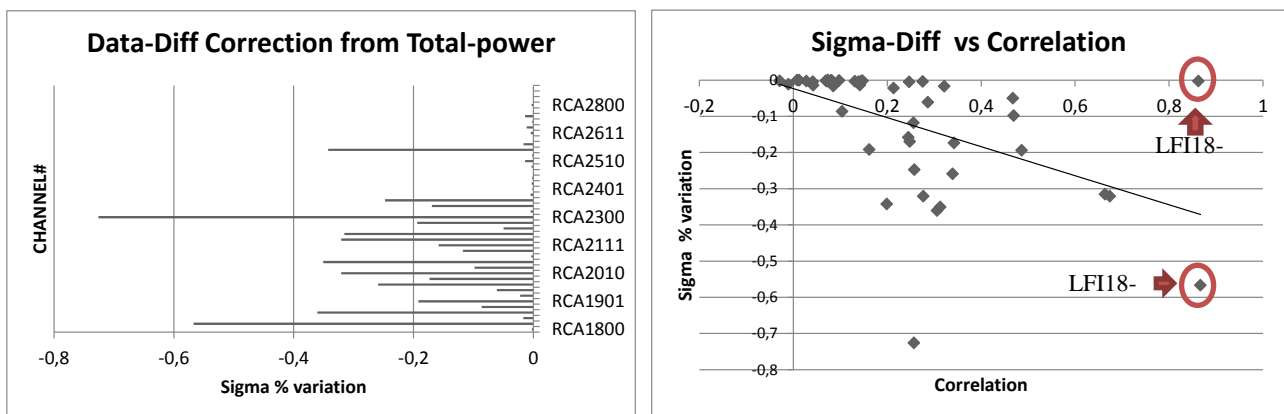
Figure 5 Left panel: Sigma variation after correction. (Channels are grouped following the sequence 00-01-10-11). Right panel: Sigma improvement calculated on diff data versus Correlation at total power level data. Highlighted by red circles the two different behaviors of LFI18-00 and LFI18-01.
