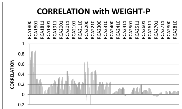
Figure 1 Linear correlation coefficient variation versus channels. Each bar is obtained stacking all the possible correlation values obtained for that channel changing the weight 'p' (causing the smoothed shape of bars)
