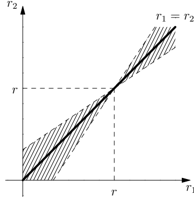
Figure 2: During the calibration of CSL data OCA2, the REBA calibration software, looked for solutions that were near the r_1 = r_2 line. Provided that r_1 \neq r_2 , these are the solutions that guarantee the best compression ratio. However, when considering flight data one has to minimize the error on the gain modulation factor r too. In order to keep its error under a desired level, the pair (r_1, r_2) must not fall within a region around the r_1 = r_2 line (the hatched region in the figure).
