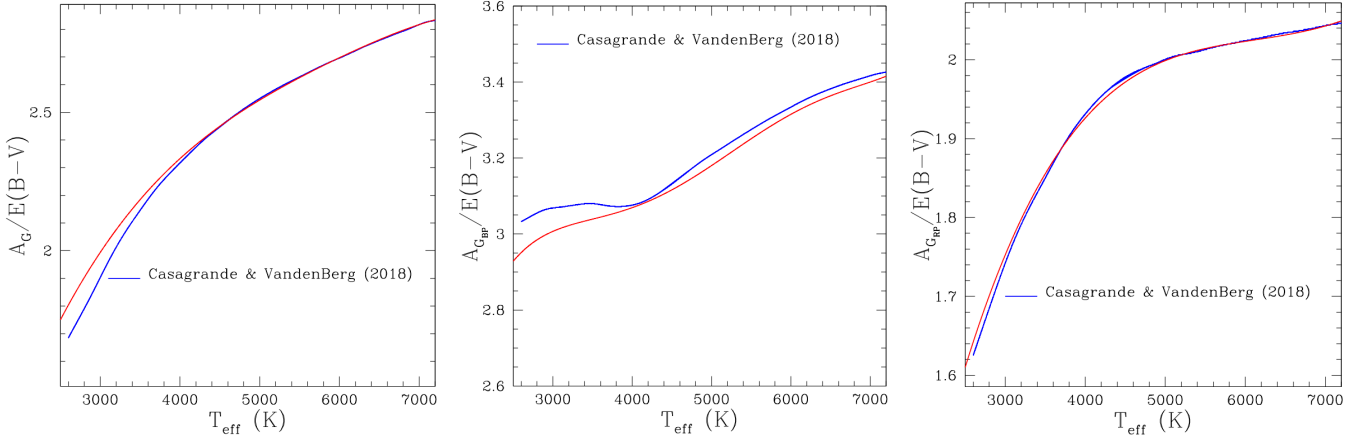
Fig. 13. Relations between A_G/E(B-V) (left), A_{GBP}/E(B-V) (middle), A_{Grp}/E(B-V) (right) and effective temperature T_{\text{eff}} derived with the procedure described in the text (Sect. 5.2). The red lines represent our interpolating relations and the blue lines models from Casagrande & Vandenberg (2018).
