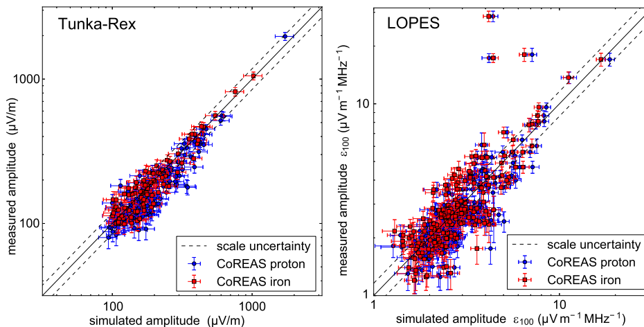
Fig. 3. Radio amplitude at each Tunka-Rex station with signal (left), and at 100 m distance from the shower axis for events measured by LOPES (right) over the amplitudes simulated by CoREAS (the left figure is slightly modified from Ref. [17]). For both experiments the standard reconstruction pipelines are used, i.e., Tunka-Rex amplitudes are the maximum absolute values of the electric-field vector in the band of 35–76 MHz, and LOPES amplitudes are the maximum of a Hilbert envelope to the east–west component in the band of 43–74 MHz.
