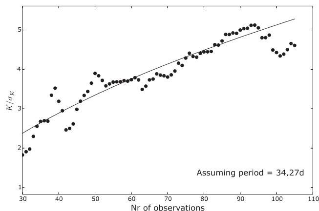
Figure 8. S/N of the semi-amplitude for a signal with a period P = 34.27 days (assuming a circular orbit) vs. number of data points. The solid line represents a square root function with y = 0.61\sqrt{x} - 0.96 (best fit to the data).
