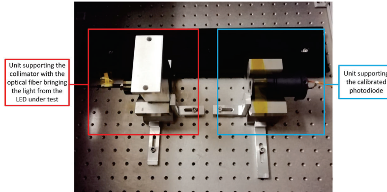
Figure 8. Setup for the calibration of the LEDs.
