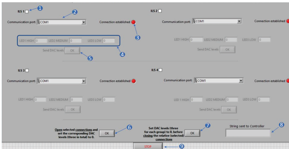
Figure 7. GUI to command the ILS LEDs.
