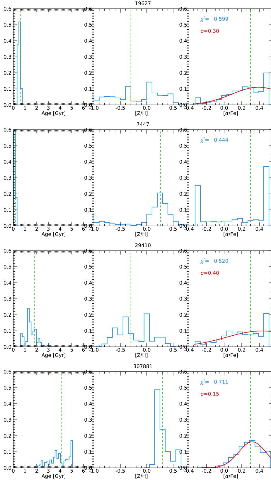
Figure A3. Mock spectra analysis: best-fitting age, metallicity, and [alpha/Fe] distributions for different sets of Lick indices as used for real data analysis (see Table 5). The vertical dashed green lines indicate the true input parameters. A Gaussian fit to the [alpha/Fe] distribution is shown in red.
