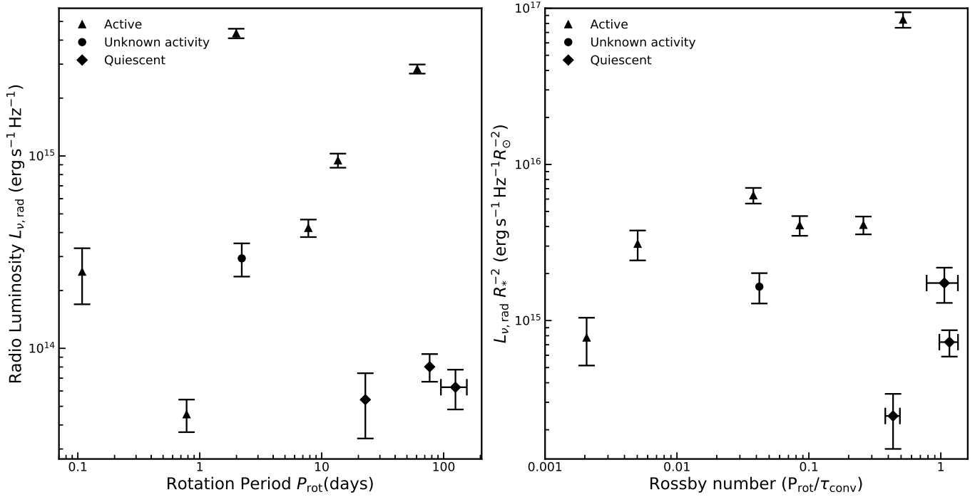
Figure 2. 144 MHz radio luminosity L_{\nu, \text{rad}} as a function of rotation period P_{\text{rot}} (left panel), and radio surface flux density ( L_{\nu, \text{rad}}/R_*^2 , where R_* is stellar radius) as a function of Rossby number R_o (right panel), for ten of our M dwarf stellar systems. Chromospherically active, quiescent, and unknown chromospheric activity stellar systems are plotted as triangles, diamonds, and circles, respectively. We find no correlation between L_{\nu, \text{rad}} and P_{\text{rot}} , or with L_{\nu, \text{rad}}/R_*^2 and R_o , with 95% confidence. The uncertainties in P_{\text{rot}} and R_o are smaller than the symbol size unless otherwise indicated. The error bars represent 1- \sigma uncertainty.
