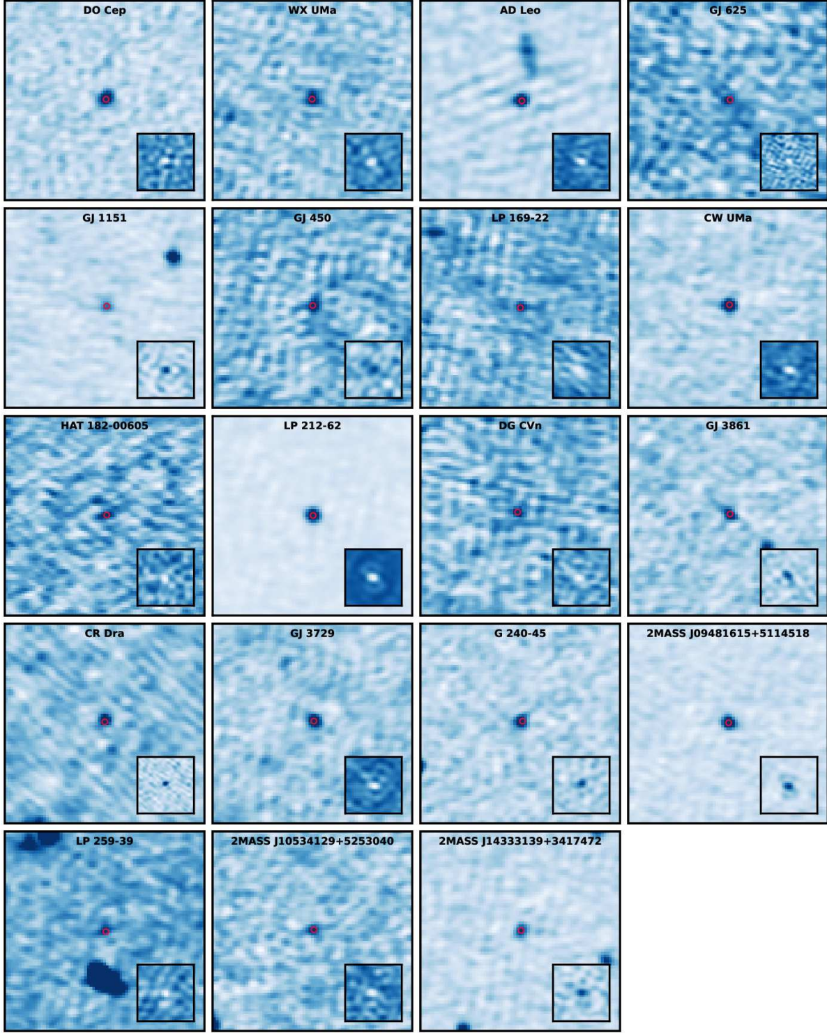
Supplementary Information Figure 1. Total intensity (Stokes I) and circularly polarised (Stokes V) (insets) 144 MHz images of the detected M dwarf systems. The red circle in each image represents the position of the Gaia DR2 counterpart at the time of the LOFAR observation. The radius of the circle is 1'' . The intensity scale of each image is different, with dark-blue representing positive flux density. All detections are \geq 4\sigma in both Stokes I and V. The Stokes I images are deconvolved and have a 5'' point-spread function. The Stokes V images are not deconvolved and have a 20'' diameter point-spread function. The horizontal and vertical axes of each image are right-ascension and declination, respectively.
