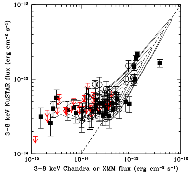
Figure 11. Comparison between the Chandra (full square symbols) or XMM-Newton (empty circle symbols) and the NuSTAR 3–8 keV fluxes. NuSTAR 90% upper limits are plotted in red as downward arrows. Black contours show the density of sources in the simulated sample when comparing 3–8 keV input fluxes and measured/deblended fluxes as in Figure 8.
