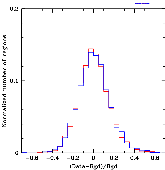
Figure 2. Normalized distributions of relative differences between counts extracted from observed data and background maps in each tile for FPMA (red) and FPMB (blue).
