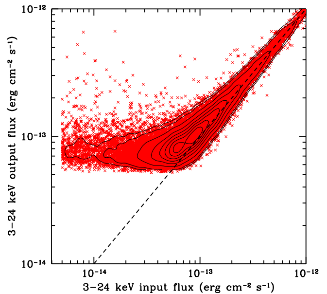
Figure 8. Comparison between 3–24 keV input fluxes and measured total fluxes in the simulations for all the sources with DET_ML above the 99% reliability threshold in the 3–24 keV band. Black contours show the source density.
