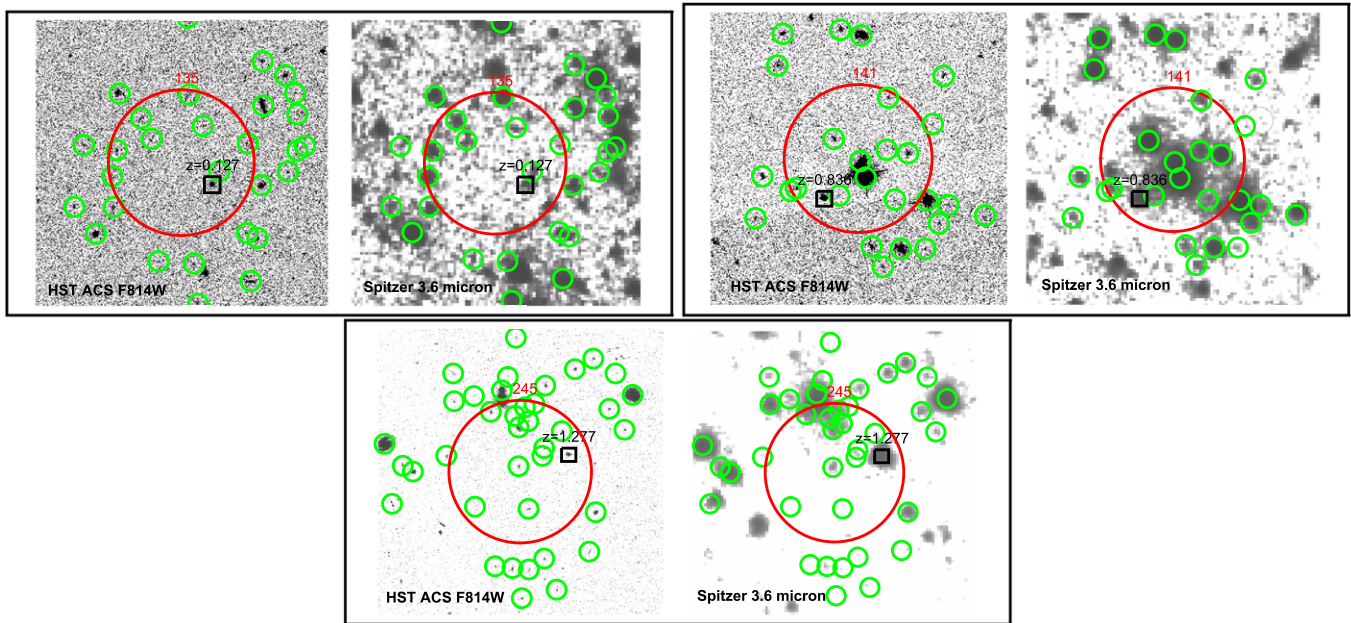
Figure 16. Postage-stamp images of the 30'' \times 30'' sky around NuSTAR sources ID 135, 141, and 245 (from top to bottom). For each source the HST ACS F814W and Spitzer IRAC (3.6 \mu\text{m} ) images are presented. Red circles = NuSTAR position; green circles = optical catalog sources; black squares = sources with spectroscopic identification.
