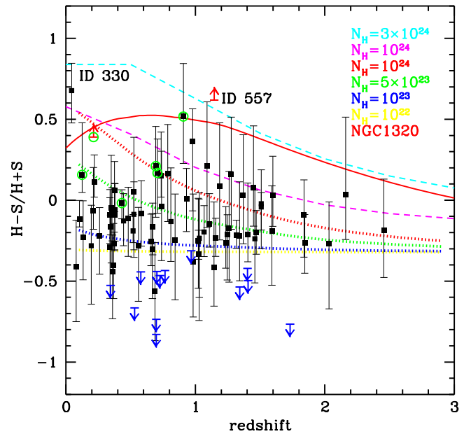
Figure 13. Hardness ratio (with 1 \sigma errors) distribution vs. redshift for all the sources matched to a Chandra or XMM-Newton counterpart. Blue downward arrows represent 1 \sigma upper limits on the HR value as computed by BEHR. Red upward arrows represent lower limits. Dotted lines show power law models with \Gamma = 1.8 , Galactic column density and intrinsic column densities of 10^{22} , 10^{23} , 5 \times 10^{23} , and 10^{24} \text{ cm}^{-2} (from bottom to top) as function of redshift. Dashed lines show the HR predicted using the more complex MYTorus model with column densities of 10^{24} and 3 \times 10^{24} \text{ cm}^{-2} (from bottom to top). The red solid line represents the HR evolution of NGC 1320 best spectral model from Baloković et al. (2014). The green circles label the candidate obscured sources by Lanzuisi et al. (2015).
