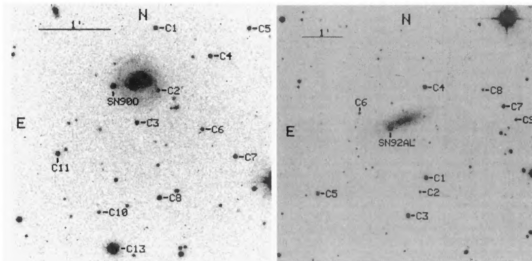
FIG. 2. V band CCD images of the two SNe Ia, 1990 and 1992al, discovered at other observatories and included in the Calán/Tololo follow-up photometric program. The photometric sequence stars are labeled along with the SNe.
