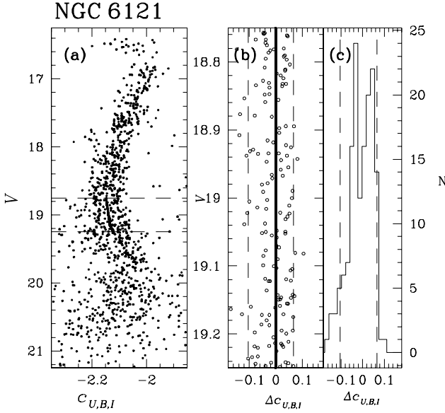
Fig. 9. Procedure to estimate the MS width for NGC 6121. Panel (a) shows the V versus c_{U,B,I} CMD of NGC 6121. The thick line is the MS fiducial line (see text for details). Panel (b) shows the verticalized MS between the two dashed lines of panel (a). Panel (c) is the distribution of the color for the stars of panel (b).
