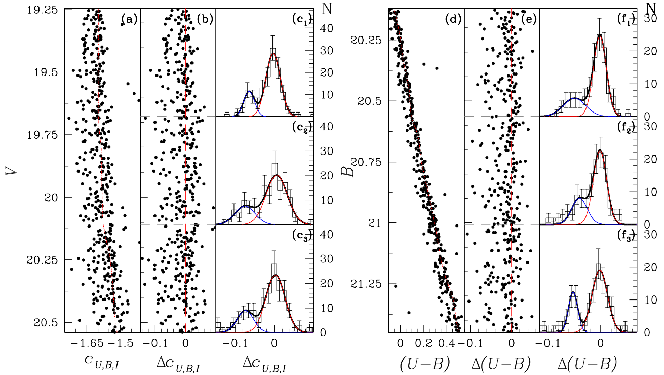
Fig. 10. Procedure to estimate the fraction of rMS and bMS stars in NGC 6752 using the V versus c_{U,B,I} diagram (panels a ), b ), and c ), and the B versus U - B CMD (panels d ), e ), and f ). Panels a ) and d ) reproduce the same diagrams as Figs. 8 and 5. The red line is the rMS fiducial line. Panels b ) and e ) show the verticalized MS. The histogram distribution of \Delta(\text{color}) for the stars of the panel b ) and e ) is plotted in panels c ) and f ) for three intervals of magnitude. The thick black lines, superimposed to each histogram, are the best-fitting biGaussian functions, whose components are colored red and blue. In the case of V versus c_{U,B,I} CMD, we found that rMS and bMS contain 77 \pm 4\% and 23 \pm 8\% of MS stars in panel c1 ), 74 \pm 5\% and 26 \pm 8\% of MS stars in panel c2 ) and, 75 \pm 5\% and 25 \pm 8\% of the MS stars, respectively. In the case of B versus (U - B) CMD, we found that rMS and bMS contain 72 \pm 5\% and 28 \pm 8\% of MS stars in panel f1 ), 74 \pm 6\% and 26 \pm 9\% of MS stars in panel f2 ), 73 \pm 5\% and 27 \pm 8\% of MS stars in panel f3 ), respectively.
