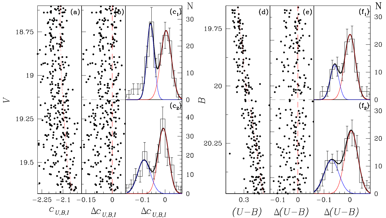
Fig. 11. As in Fig. 10, in the case of NGC 6121. In the case of V versus c_{U,B,I} CMD, we found that rMS and bMS contain 60 \pm 7\% and 40 \pm 8\% of MS stars in panel c1 ), 61 \pm 6\% and 39 \pm 7\% of MS stars in panel c2 ), respectively. In the case of B versus (U - B) CMD, we found that rMS and bMS contain 67 \pm 7\% and 33 \pm 10\% of MS stars in panel f1 ), 75 \pm 13\% and 25 \pm 14\% of MS stars in panel f2 ), respectively.
