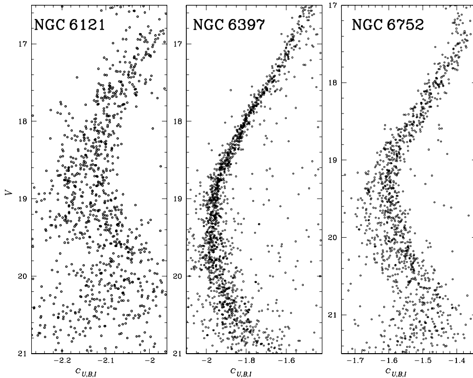
Fig. 8. V , c_{U,B,I} diagrams for NGC 6121 ( left ), NGC 6397 ( middle ), and NGC 6752 ( right ).
