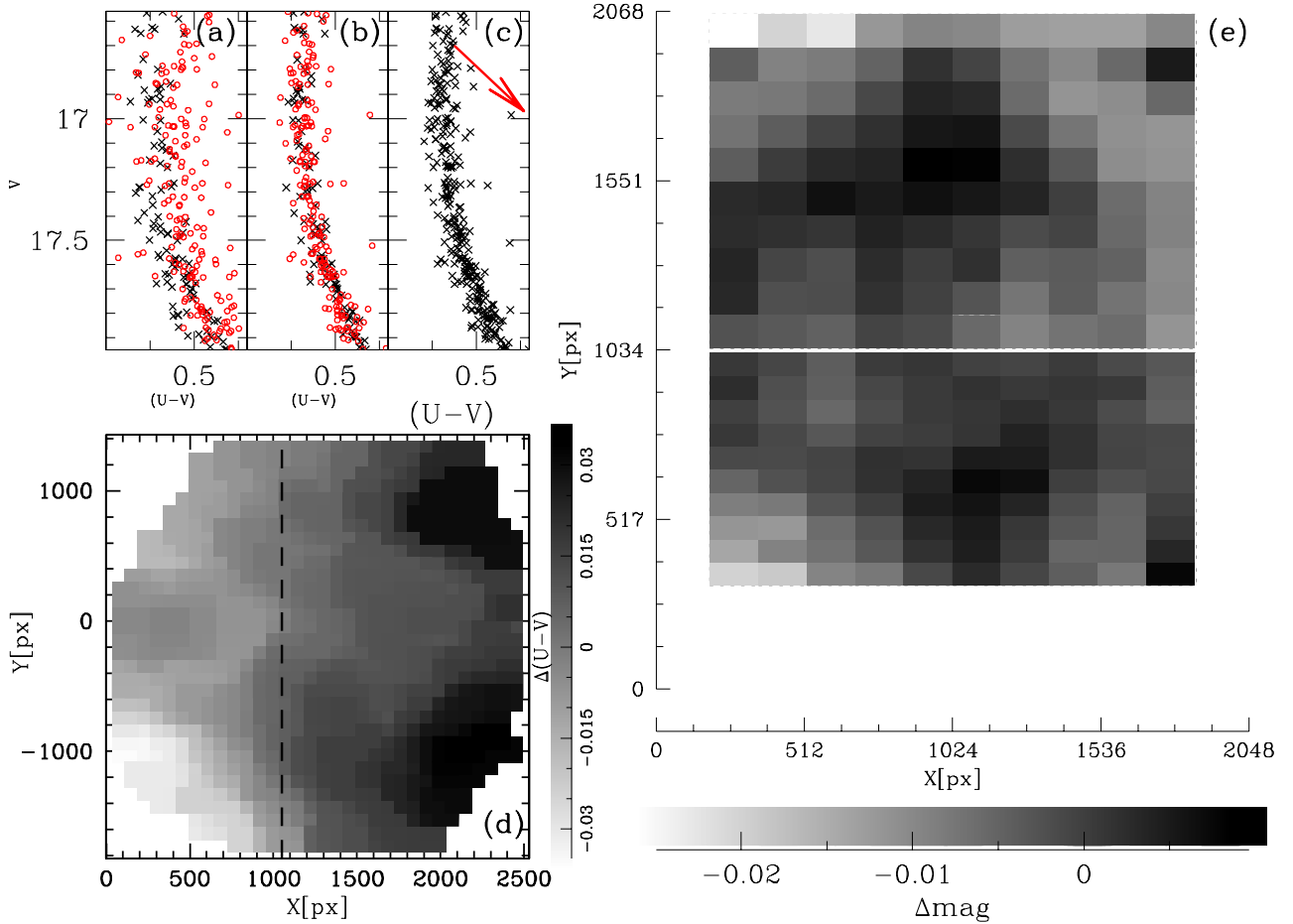
Fig. 3. Visualization of the effects of the photometric zero-point variation. Panel a): CMDs zoomed into the MS region of NGC 6397 before the zero-point correction; panel b): CMD after the zero-point correction; panel c): CMD after the differential reddening correction (in red the reddening vector, scaled by a factor 1/3); panel d): map of the color zero-point variation; the dashed line divide the two groups of stars shown in the panels a) and b); panel e): final \Delta\text{mag} correction grid for the filter v_{\text{HIGH}} and the NGC 6397 data set.
