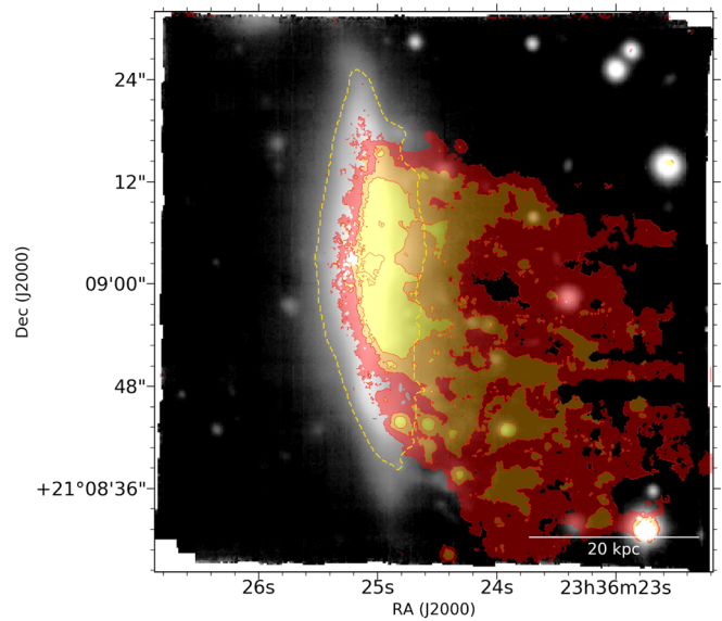
Figure 1. MUSE white light image of JW100, overlaid with the contours of the H \alpha emission (the filled area) and the stellar continuum (the gold dashed line), as defined in Gullieuszik et al. (2020).
