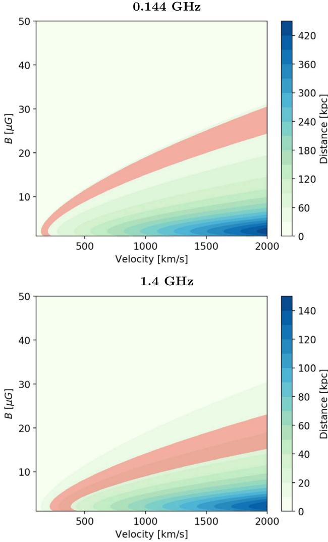
Figure 7. Cooling length parameter spaces for the radio tail observed at 0.144 GHz (top) and 1.4 GHz (bottom). The red regions correspond to the observed projected lengths, which are here reported with a 6 kpc uncertainty due to the current resolution of 12".
