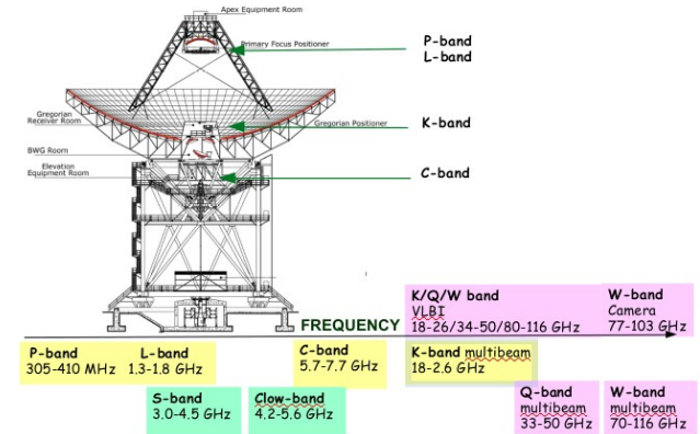
Figure 1. Receivers of the Sardinia Radio Telescope and their focal position: current (yellow), under construction (green) and those expected from the PON project (pink).
