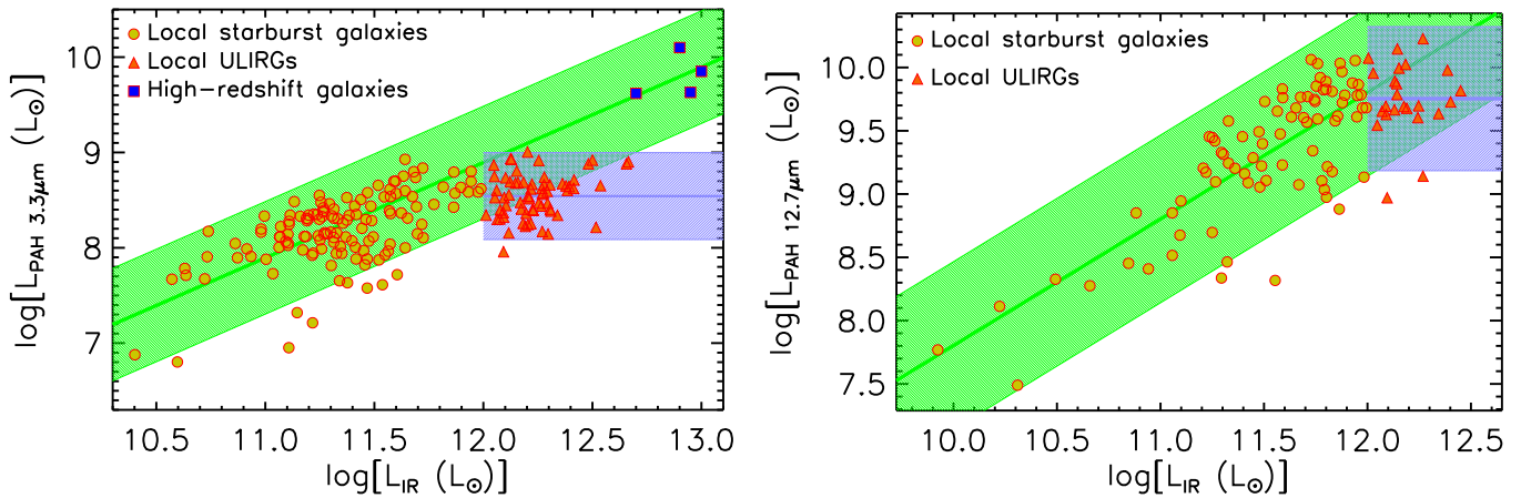
Figure 3. Luminosity of the PAH 3.3\ \mu\text{m} (left)/PAH 12.7\ \mu\text{m} (right) line vs. continuum IR luminosity. The green bands show the 2\sigma range around the mean linear relation \log(L_\ell) = \log(L_{\text{IR}}) + c for local star-forming galaxies with L_{\text{IR}} < 10^{12} L_\odot (circles) and high-redshift galaxies (squares; only for PAH 3.3\ \mu\text{m} line, data of high- z sources were available); the derived value of c \equiv \langle \log(L_\ell/L_{\text{IR}}) \rangle is -3.11 \pm 0.30 (for PAH 3.3\ \mu\text{m} ) and -2.20 \pm 0.33 (for PAH 12.7\ \mu\text{m} ). The azure bands show the 2\sigma spread around the mean line luminosity for the sample of local ULIRGs (triangles) whose line luminosities appear to be uncorrelated with L_{\text{IR}} ; the mean line luminosity \langle \log(L_\ell) \rangle of these objects is 8.54 \pm 0.23 (for PAH 3.3\ \mu\text{m} ) and 9.75 \pm 0.28 (for PAH 12.7\ \mu\text{m} ).
