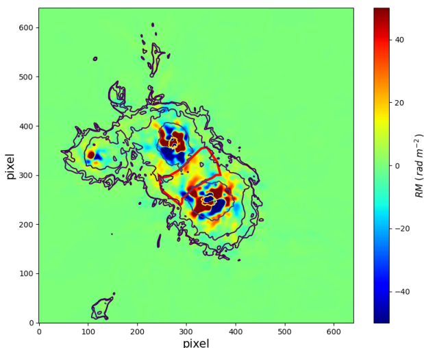
Fig. 11. Faraday depth map obtained using the cluster simulation (Witior et al. 2019a) - see text for details. The contours are from the density field in Fig. 10, and the selected bridge region is highlighted in red. Every pixel is \sim 16 kpc long.
