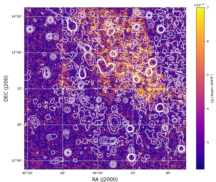
Fig. 3. Slice of the FDF cube at \phi \sim 7.5 \text{rad m}^{-2} showing the Galactic polarised emission detected in the field. Total intensity is overlaid with contours at 4, 20, 40, 80 \times \text{RMS} taken from Fig 1.
