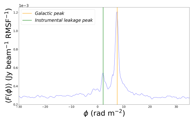
Fig. 4. Faraday depth amplitude averaged over all the lines of sight within the bridge region at 107'' resolution. It displays two peaks, which are due to the Galactic foreground medium and the instrumental leakage respectively.
