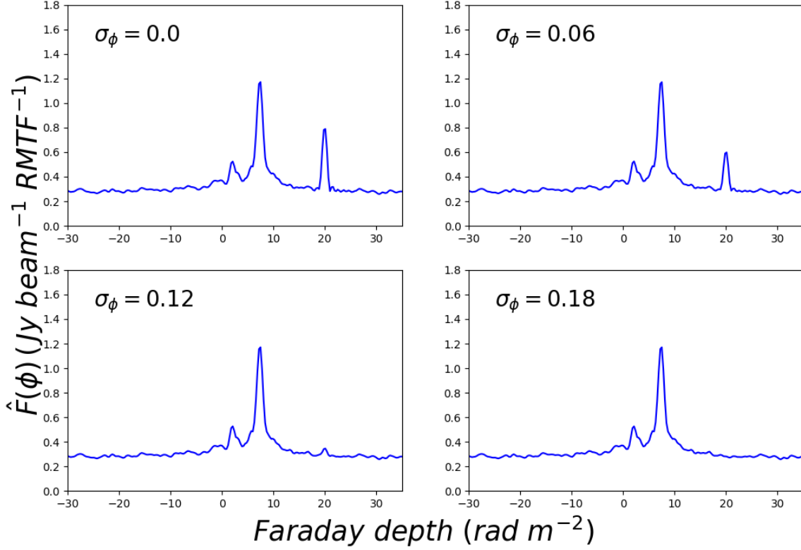
Fig. 8. Examples of FDFs of the bridge region as a function of Faraday dispersion \sigma_\phi , after injection of the depolarisation model in the data - see text for details. The peak at 20 rad m -2 decreases until it completely disappears below the nose for the \sigma_\phi = 0.18 rad m -2 model.
