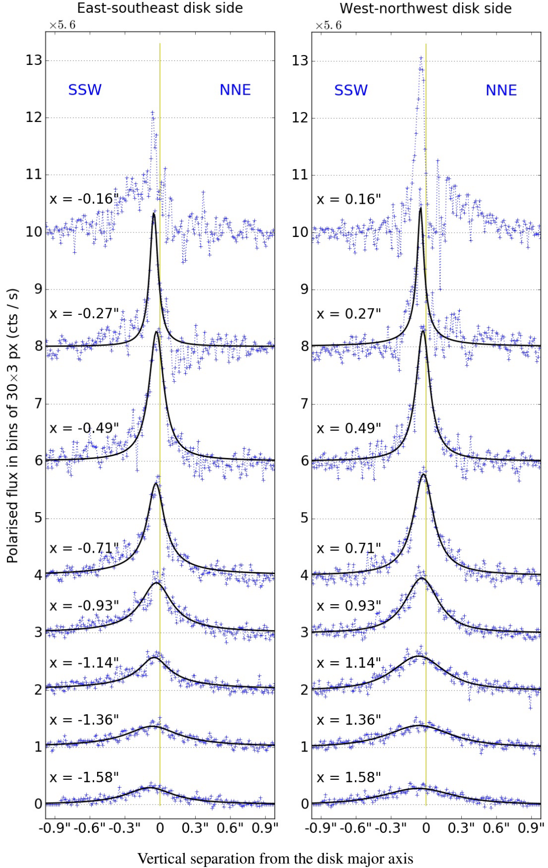
Fig. 5. HIP 79977 polarized intensity cross-sections perpendicular to the disk major axis at several separations x from the central star. Blue crosses are the data from the 30 \times 3 px binned Q_p image. Black solid lines show the Moffat profile fits to the data except for x = \pm 0.16'' , where the data are unreliable because of systematic effects. The cross-sections are offset vertically by integer units for clarity. The yellow line marks the position of the disk axis.
