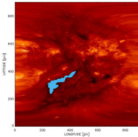
(a) Example of AIA 193 Å ROI (blue region) identifying a mid-latitude CH. (02-03-2012 18:00:00)
