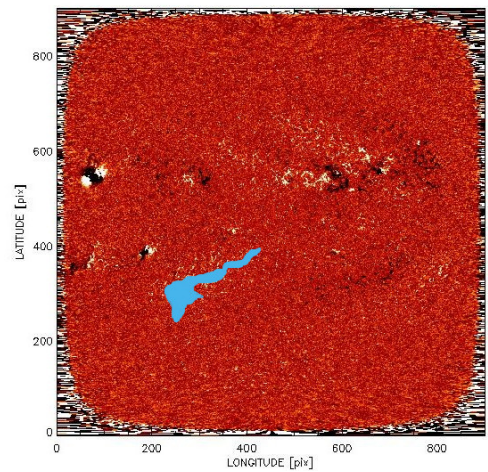
(b) The same ROI superposed onto HMI magnetogram. (02-03-2012 18:00:00)
