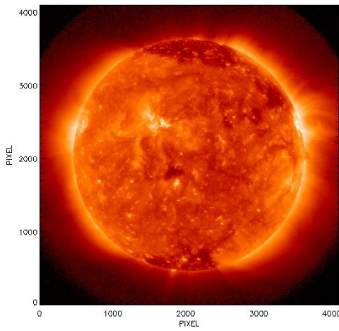
(a) AIA 193 Å image before limb brightening removal. (06-25-2017 18:00:00)
