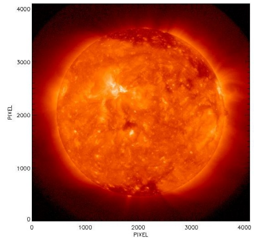
(b) AIA 193 Å image after limb brightening removal. (06-25-2017 18:00:00)
