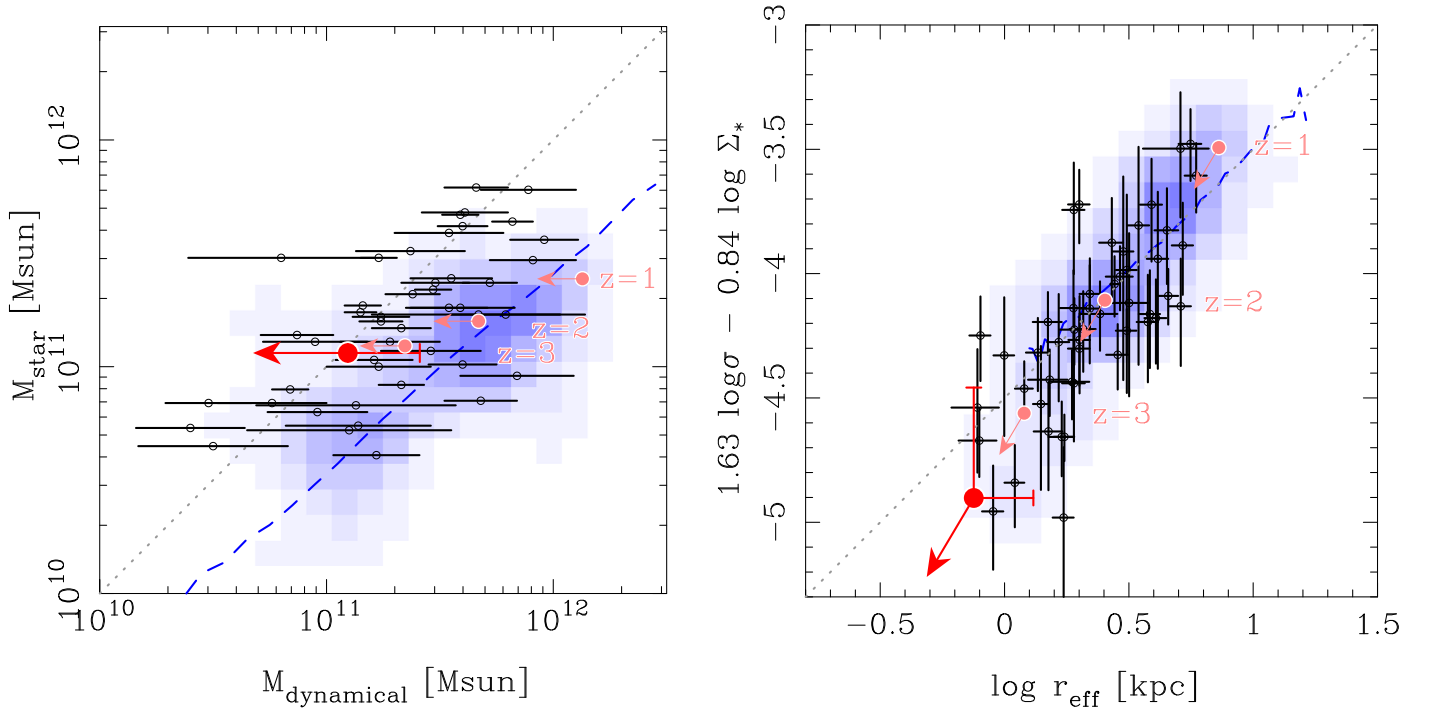
Figure 5. Left: stellar mass plotted against dynamical mass. The dotted line shows M_{*} = M_{\text{dyn}} . The black points are the lower redshift objects ( z \sim 2 ) as in Figure 4. The shades are quiescent galaxies from LEGA-C, and the dashed curve is the running median of the distribution of quiescent galaxies with \text{sSFR} < 10^{-10} M_{\odot} \text{ yr}^{-1} drawn from SDSS DR15 (Aguado et al. 2019). SFR and stellar mass are from Granada FSPS fits (Ahn et al. 2014). The red point is the z = 4 object. The pink points are the expected evolutionary track assuming constant velocity dispersion (see the text for details). Right: mass fundamental plane. The dotted line is a fit from Bezanson et al. (2013). The other symbols are the same as those in the left panel.
