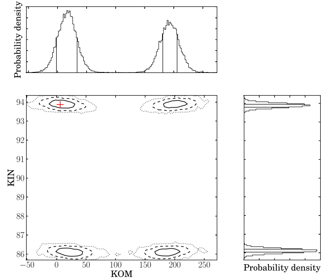
Figure 11. Same caption as Fig. 9 for PSR J1909–3744.
