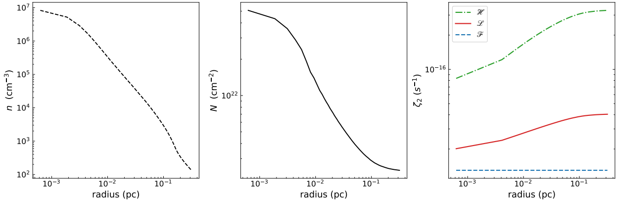
Fig. 1. Left panel: H 2 volume density profile ( n ) in the physical model of L1544. Central panel: column density profile. Right panel: \zeta_2 profiles for the \mathcal{F} (dashed blue curve), \mathcal{L} (solid red), and \mathcal{H} (dashed-dotted green) models. The profiles for the models \mathcal{L} and \mathcal{H} PI18 have been derived integrating the volume density profile of the core model to obtain the column density profile, and then using the relation between \zeta_2 and N .
