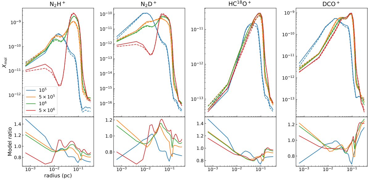
Fig. 11. Top panels: abundance profiles obtained from the model \mathcal{L} (solid lines), and from the model with constant \zeta_2 = 3 \times 10^{-17} s^{-1} (dashed lines). The different colours refer to the four time steps investigated in this work (labelled in the first panel , in year). Bottom panels: ratios between the abundance profiles from model \mathcal{L} and from the model with constant \zeta_2 = 3 \times 10^{-17} s^{-1} . The colour code is the same as for the upper panels.
