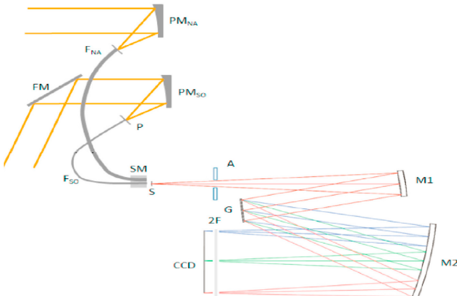
Fig. 1. Schematics of the UVIS instrument reproduced from [Vandaele et al., 2015]: the entrance optics for nadir observations (NA) with the parabolic mirror ( PM_{NA} ) and the bundle of fibers ( F_{NA} ), the entrance optics for solar occultation observations (SO) with the flat mirror (FM) located in the periscope, the parabolic mirror ( PM_{SO} ), the pinhole (P) and the optical fiber ( F_{SO} ); the selector mechanism (SM); the spectrometer with the entrance slit (S), the aperture (A), the collimating mirror (M1), the diffraction grating (G), the focusing mirror (M2), the 2nd order filter (2F) and the detector (CCD).
