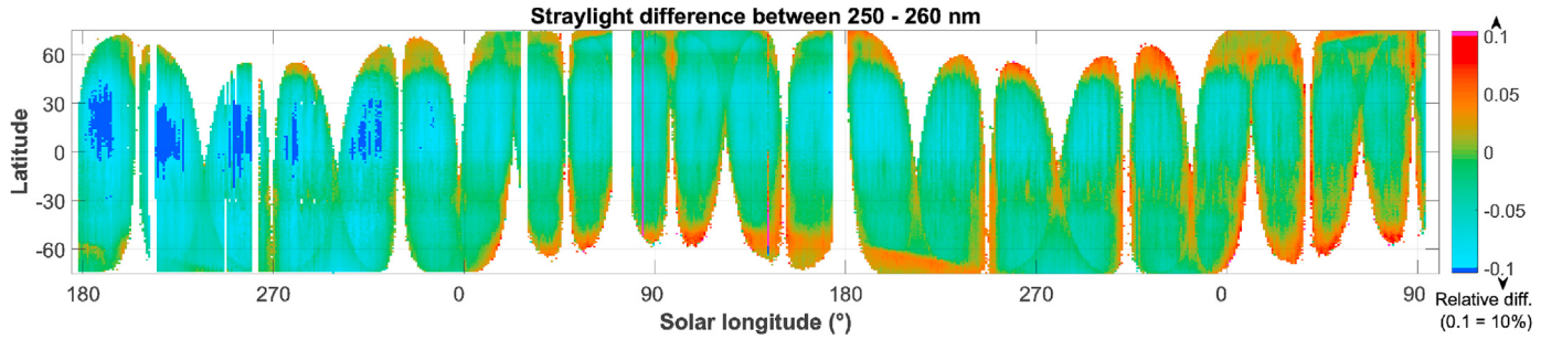
Fig. 11. Relative difference between the straylight estimation of the two methods between 250 and 260 nm for the period going from May 2018 to end of August 2021. The values < -10\% are represented in dark blue and > 10\% in magenta.
