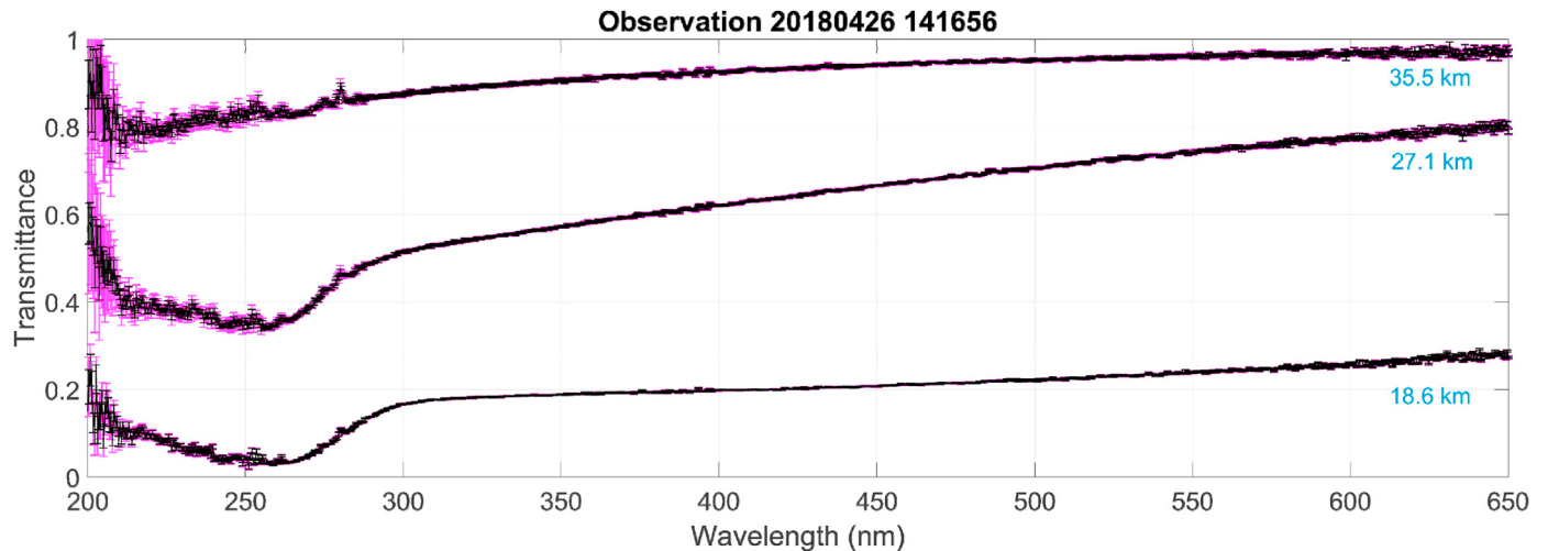
Fig. 16. Example of occultation spectra in transmittance with errors (same observation as in Fig. 12). The black curve gives the “random” error while the purple curve also includes the 5% straylight error (i.e. “total” error).
