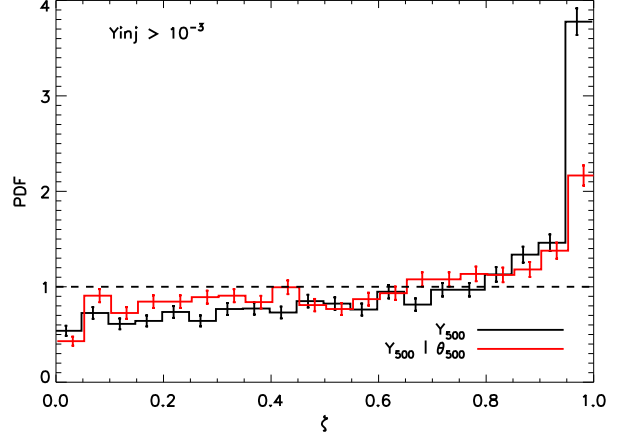
Fig. 14. Bounded probability histograms, as in the top panel of Fig. 13, but for the converted p(Y_{500}) marginal and p(Y_{500}|\theta_{500}) sliced posteriors.
