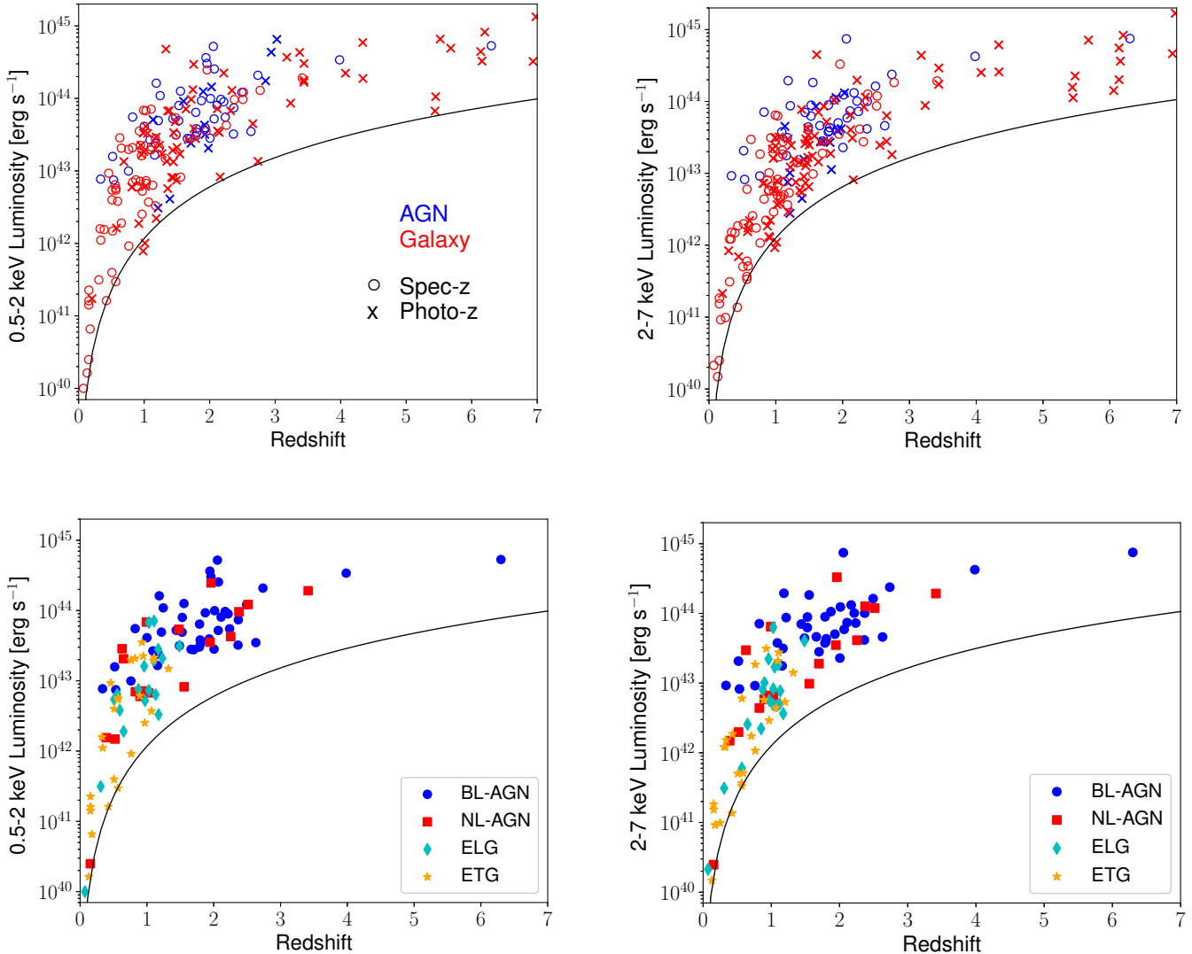
Fig. 11. Top: Intrinsic, absorption-corrected luminosity in the 0.5–2 keV (left) and 2–7 keV (right) band as a function of redshift. Sources with a spectroscopic redshift are plotted with circles, while sources with only a photometric redshift are plotted with crosses. Sources with a BL– or NL-AGN spectrum or with a SED best-fitted with an AGN template are plotted in blue, while sources with a ETG or ELG spectrum, or with a SED best-fitted with a galaxy template are plotted in red. We also plot as a black solid line the luminosity corresponding to the flux at which 10% of the field is covered. Bottom: same as above, but for the spectroscopic subsample alone. BL-AGNs are plotted as blue circles, NL-AGNs as red squares, emission line galaxies as cyan diamonds, and early type galaxies as orange stars.
