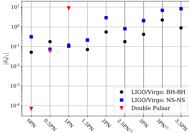
FIG. 7. Update of Fig. 6 in Ref. [178] (including data from Refs. [180,181]), which shows the 90% upper bounds on the absolute magnitude of the GR violation parameters \delta\hat{\phi}_i , from 0PN through 3.5PN (“relative” order) in the inspiral phase (see, e.g., Ref. [182] for the definition of the PN phase coefficients and Ref. [178] for further details on the method). As discussed in Ref. [178], the 0.5PN parameter is zero in GR and, therefore, understood not as a relative but as an absolute shift. Black circles show the combined limits from the double BH mergers, blue squares are the limits from the double-NS merger GW170817, and red triangles give the limits derived from the double pulsar GW test in this paper. The PN order on the x axis is in the GR radiation reaction, where the leading contribution (0PN) corresponds to the dissipative 2.5PN term in the equations of motion. Note that such a comparison of tests with different compact objects (BHs vs NSs) as well as different gravity regimes (mildly relativistic vs highly relativistic strong field) does come with a caveat, which is explained in more detail in the text.
