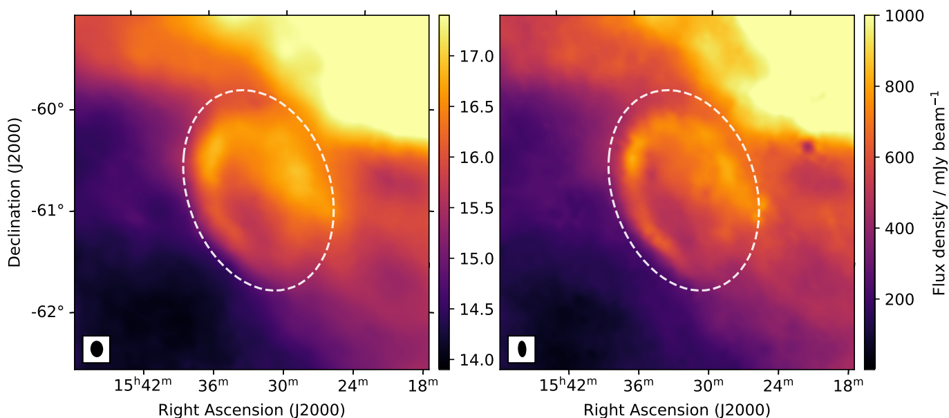
Fig. 2. 3:5 \times 3:5 of the region surrounding G321.3–3.9 as seen at 1.4 GHz by CHIPASS (left panel) and at 2.3 GHz by S-PASS (right panel). The panels show the region after the conversion from K to \text{Jy beam}^{-1} and the subtraction of point sources. The dashed line highlights the area within which the SNR is located.
