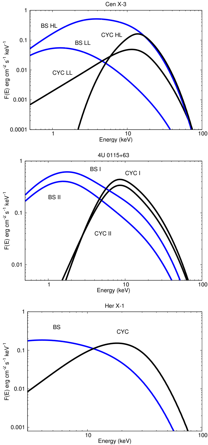
Fig. 4. From top to bottom : componentized bremsstrahlung and cyclotron spectra of Cen X-3, 4U 0115+63, and Her X-1 obtained from the best-fit models given in Table 2.
