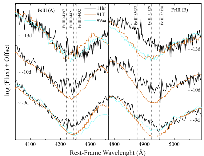
Figure 9. Absorption lines of Fe III in the spectra of SN 2011hr, SN 1991T, and SN 1999aa at early phases. The positions of these lines at a velocity of 12,000 \text{ km s}^{-1} are marked to guide the eyes.
