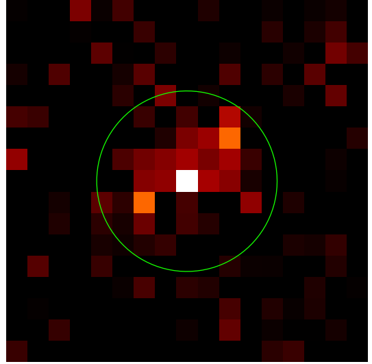
Fig. 7. Stacked X-ray image at the position of the centrals (excluding individual detections), from the combined Chandra and XMM-Newton 0.5–2 keV image of the COSMOS field. For reference, the green circle has a radius of 15".
