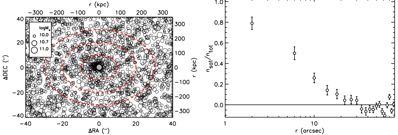
Fig. 3. Left: positions of all satellite candidates (open circles) compared to their respective centrals (filled circle), with the overdensity most visible at \leq 10'' . The size of each symbol varies as a function of its stellar mass. The red dashed contours show scales of 10'' , 20'' , and 30'' , respectively. Right: fraction of expected “real associations” among satellite candidates, n_{\text{sat}}/n_{\text{tot}} as a function of radius (where n_{\text{sat}}(r) = n(r) - n_b , n(r) and n_b being, respectively, the number density of satellite candidates at radius r and at >50'' ).
