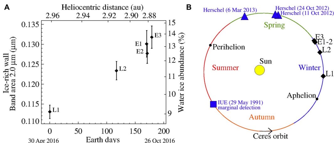
Fig. 4. Modeled increase of water ice on the crater wall and contextualization along Ceres' orbit. (A) Left axis: Band area at 2.0 \mu\text{m} calculated after isolation of the signal of the ice-rich wall by removal of the outer signal from average spectrum. Right axis: Water ice abundance as retrieved by the model (table S2). Both quantities are shown as a function of Earth days by setting the day of the first observation (L1) equal to 0. Error bars are estimated as discussed in the Supplementary Materials. au, astronomical unit. (B) Ceres orbit with International Ultraviolet Explorer (IUE) and Herschel water detections (12, 13). The orbit segment associated with the Juling observations indicates an increasing solar flux in the southern hemisphere of Ceres, where Juling is located.
