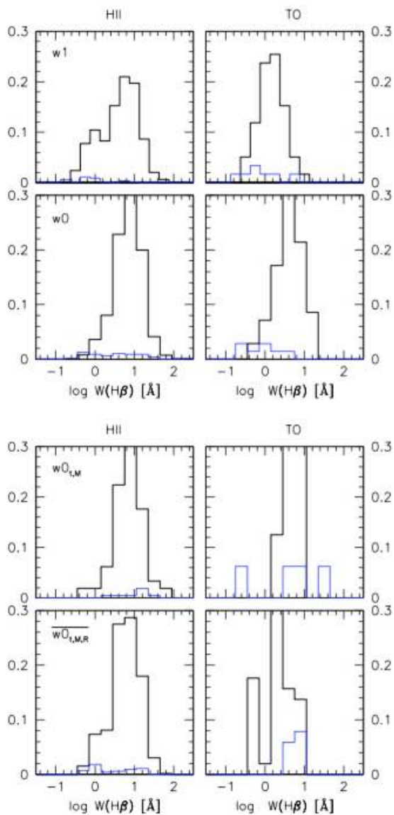
Fig. 6. Distribution of W(\text{H}\beta) (in \text{\AA} ) for sources classified as HII (left), and TO (right), for w1, w0, one realization of w0_{t,M} and w0_{t,M,R} (from top to bottom). The black histograms trace the distribution of detections, the thin blue ones the distributions of upper limits.
