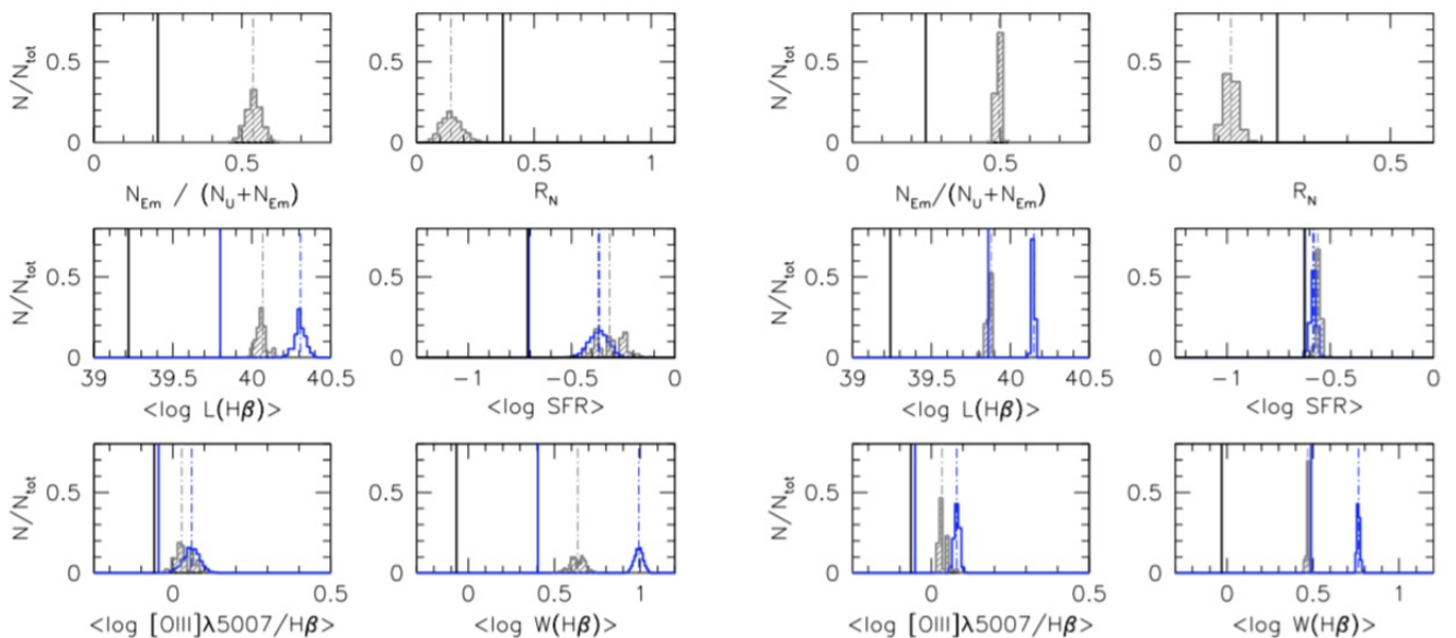
Fig. 5. Results of bootstrap simulations. The w1 sample is compared with 1000 virtual w_{0,t,M} CSs of \approx 350 sources (six leftmost panels), and with 200 virtual \overline{w}_{0,t,M,R} (six rightmost panels). The panels show median values measured for the cluster members (thick solid lines) along with the distributions of the bootstrapped sample w_{0,t,M} medians (left) and \overline{w}_{0,t,M,R} (right) and their medians (dot-dashed lines). Top: ratio R_{Em} (left), ratio R_N (from DD_{[NII]} ; right), for the revised classification (grey). The middle panels show the luminosity of H\beta in \text{erg s}^{-1} (left), and the SFR in M_{\odot} \text{ yr}^{-1} (only for HII sources; right). Blue histograms and lines refer to average values of detections only, grey histogram and lines show medians and include upper limits. Bottom panel: distributions for [OIII]\lambda 5007/H\beta (left) and W(H\beta) (right), with the same meaning of color coding.
