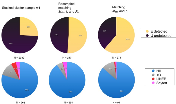
Fig. 3. Top: fractions of quiescent galaxies (black), and ELGs (yellow), for w1 cluster galaxies (left), one realization of w0_{t,M,R} and w0_{t,M} (middle and right). Bottom: prevalence of different ELG classes identified in the DD [NII] from uncensored diagnostic ratios: HII (blue), transition objects (pale grey), LINERs (red) and Seyferts (magenta), ordered as in the top row.
