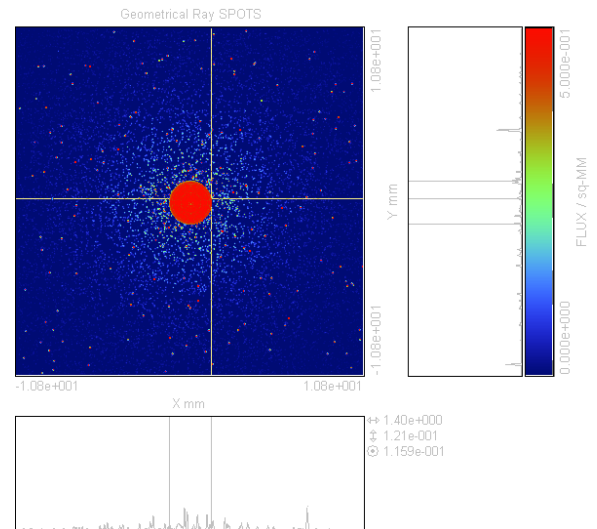
Figure 18: Extended source image with scattered light enhanced.
