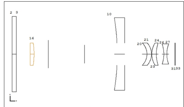
Figure 16: HRIC surfaces layout for ghost analysis.
