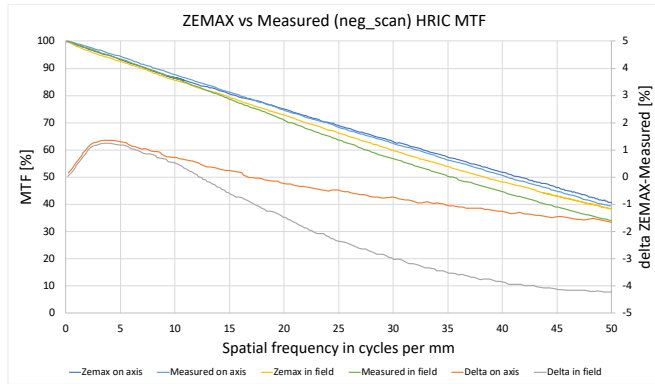
Figure 13: Diffraction MTF curves (by design vs. measured one).
