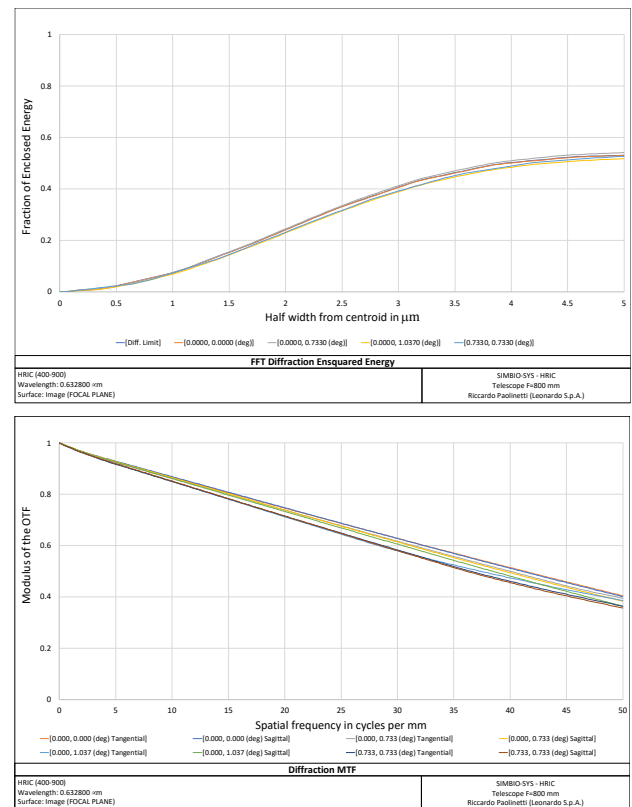
Figure 12: Fraction of EE (above) and Diffraction MTF curves at 632.8 nm (below) for the optical design.
