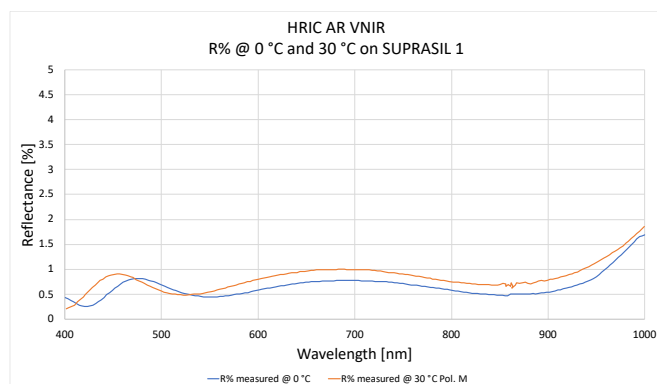
Figure 4: Corrector lenses manufactured coating curves at 0° and 30° AOI.
