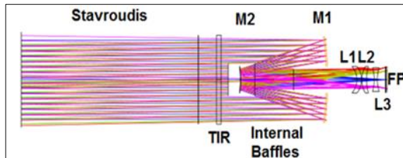
Figure 1: HRIC optical layout with TIRD filter (TIR), the two mirrors (M1 and M2), three-lens (L1, L2 and L3) corrector plus filters deposited on the detector window (FP).
