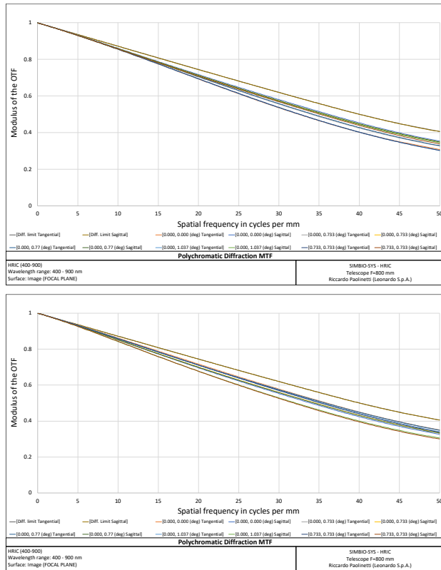
Figure 17: Polychromatic tangential and sagittal MTF at -20°C (above) and +50°C (below) in the centre and at the edge of FoV. The black curve is relative to the diffraction limited while the colored curves are relative to some points of FoV from the line of sight to the maximum FoV.
