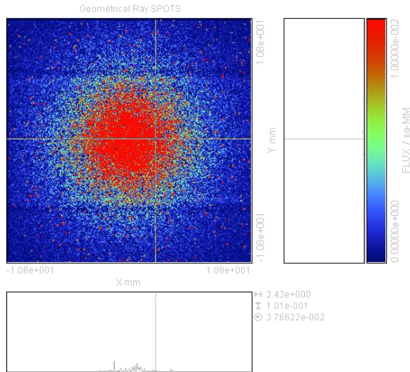
Figure 19: Straylight due to contamination 400nm.
