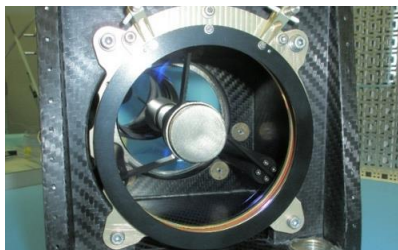
Figure 5: HRIC Camera front view, with TIRD filter (dark grey disk) before secondary mirror support.
