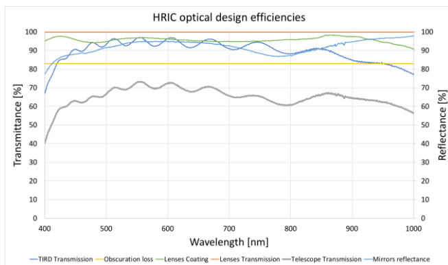
Figure 8: HRIC Optics reflectance/transmission efficiencies.
