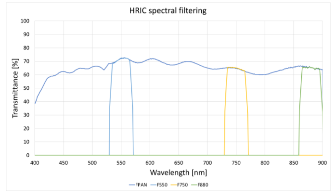
Figure 9: HRIC global optical transmission for all the spectral filters in panchromatic range (i.e., 400-900 nm).
