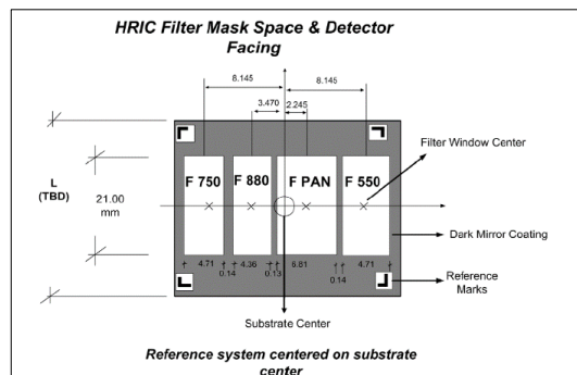
Figure 7: Filter strips dimension specification for manufacturing (view from top).
