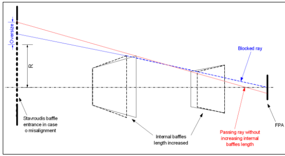
Figure 11: HRIC Internal baffles design modification to prevent stray light.
