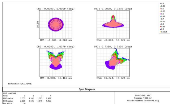
Figure 14: Spot diagrams on the image plane.
