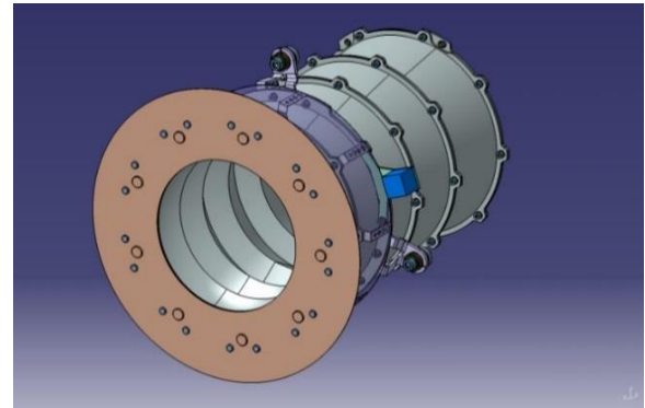
Figure 10: HRIC external baffle cad design.
