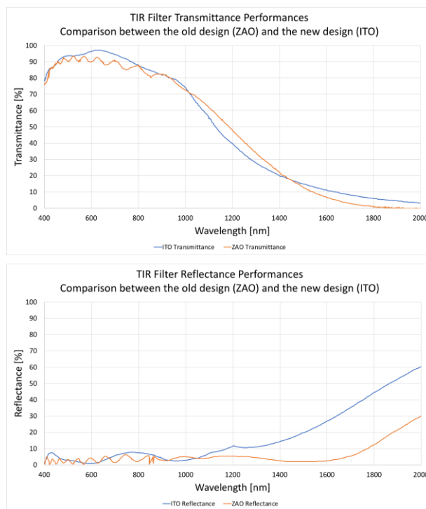
Figure 6: Comparison between ZAO and ITO transmission (above) and reflection (below) profile considered for the TIRD.
