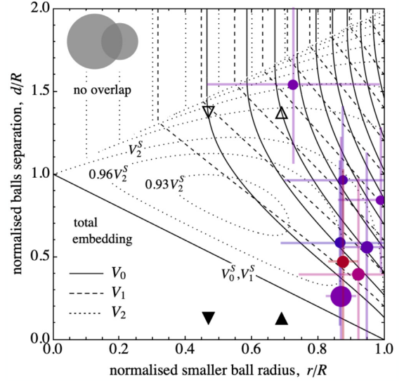
Figure 2. Minkowski functionals iso-contours for major mergers, V_\mu^{\mathcal{M}} (equations 3), as function of the smaller ball radius r and distance d from the major ball with radius R . Volume (solid lines), surface (dashed), and integrated mean curvature (dotted) levels increase by 10 per cent moving top right-hand side from the lower values attained for a single ball, V_\mu^S (for V_2^{\mathcal{M}} , also the contours corresponding to 93 and 96 per cent of V_2^S are shown). The lower (‘total embedding’) and upper (‘no overlap’) triangular regions account for trivial morphologies of one and two isolated balls, respectively. Points indicate major mergers from the LC 2 cluster catalogue (Serenio 2015, colour-coded by redshift as in Fig. 1, size proportional to R_{200c} ). Filled (empty) symbols designate a merging subclump at the pericentre (splashback) for a system at z = 0.3 ; see Table 1.
