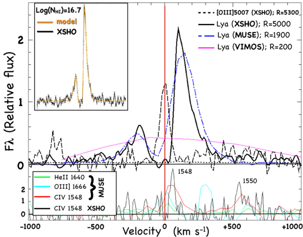
Figure 3. Comparison of the most relevant spectral features in the velocity space. Top panel: the Ly \alpha line profile is shown for different instruments (VIMOS, MUSE, X-Shooter). The [O III] \lambda 5007 emission line identified with X-Shooter is shown with a dashed line and marks the assumed systemic velocity (it has been multiplied by a factor of four for graphic purposes). Both components of the Ly \alpha line are clearly resolved at the X-Shooter spectral resolution. The inset shows an example of Ly \alpha modeling (orange line). Bottom panel: the high-ionization emission lines (as indicated in the legend) are also shown with respect to the systemic velocity. Among them, the only feature showing a significant velocity offset is the C IV \lambda 1548, 1550 doublet, with d\nu = +50 km s ^{-1} .
