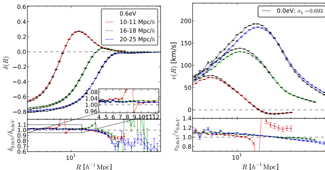
Figure 13. Left panel: matter density profile. Right panel: radial velocity profile. In both cases colored lines show the profiles for the \sum m_\nu = 0.6 \text{ eV} cosmology, whereas black lines indicate \Lambda\text{CDM} cosmology with the same \sigma_8 of the massive neutrino case, when it is computed using the total matter density field. The bottom panels show the ratios between the results from the two cosmologies.
