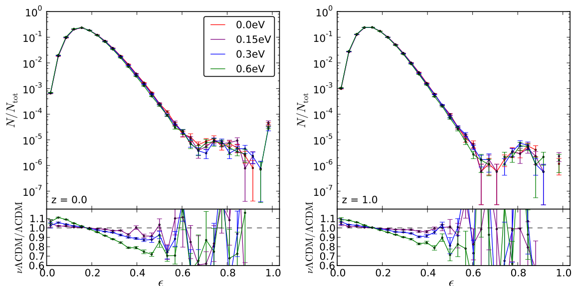
Figure 2. Number of voids with a given ellipticity, normalized by the total number of voids. The top panels show results from different cosmologies: red line is the \Lambda\text{CDM} cosmology, purple, blue and green lines correspond to \sum m_\nu = 0.15 eV, \sum m_\nu = 0.3 eV and \sum m_\nu = 0.6 eV cosmologies. The bottom panels show the ratio between the same quantity in a massive and a massless neutrino cosmologies. Left and right plots display results at redshift z = 0 and z = 1 , respectively.
