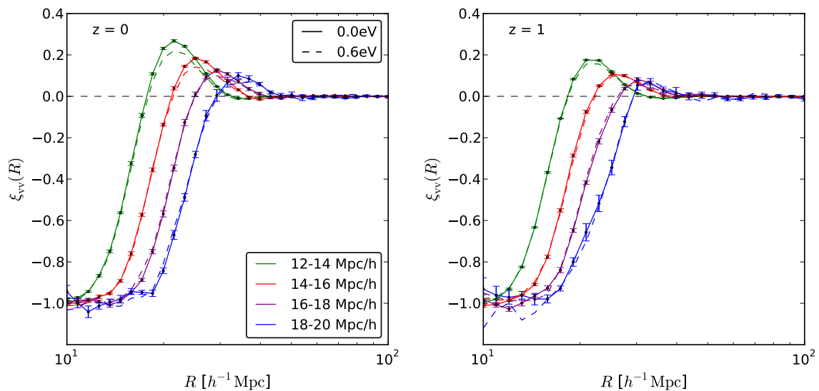
Figure 3. Two-point correlation function of voids with an effective radius in a given range. Solid lines show the results for the \Lambda\text{CDM} cosmology whereas the dashed lines indicate the results for the \sum m_\nu = 0.6 eV cosmology; different colors are related to different bins in the void radii as reported in the legend. Left and right plots display results at redshift z = 0 and z = 1 , respectively.
