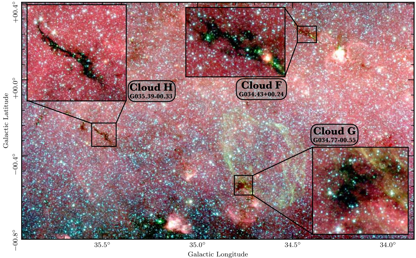
Figure 1. A three colour image of the Galactic plane where several infrared dark clouds (IRDCs) can be seen as dark extinction features. In this image, red is 8\ \mu\text{m} , green is 5.8\ \mu\text{m} , and blue is 4.5\ \mu\text{m} emission from the Spitzer GLIMPSE survey (Carey et al. 2009). Labelled are three IRDCs that are investigated within this work: Clouds F, G, and H (or G034.43 + 00.24, G034.77-00.55, G035.39-00.33). The panels show zoom-ins of these IRDCs for more detail.
