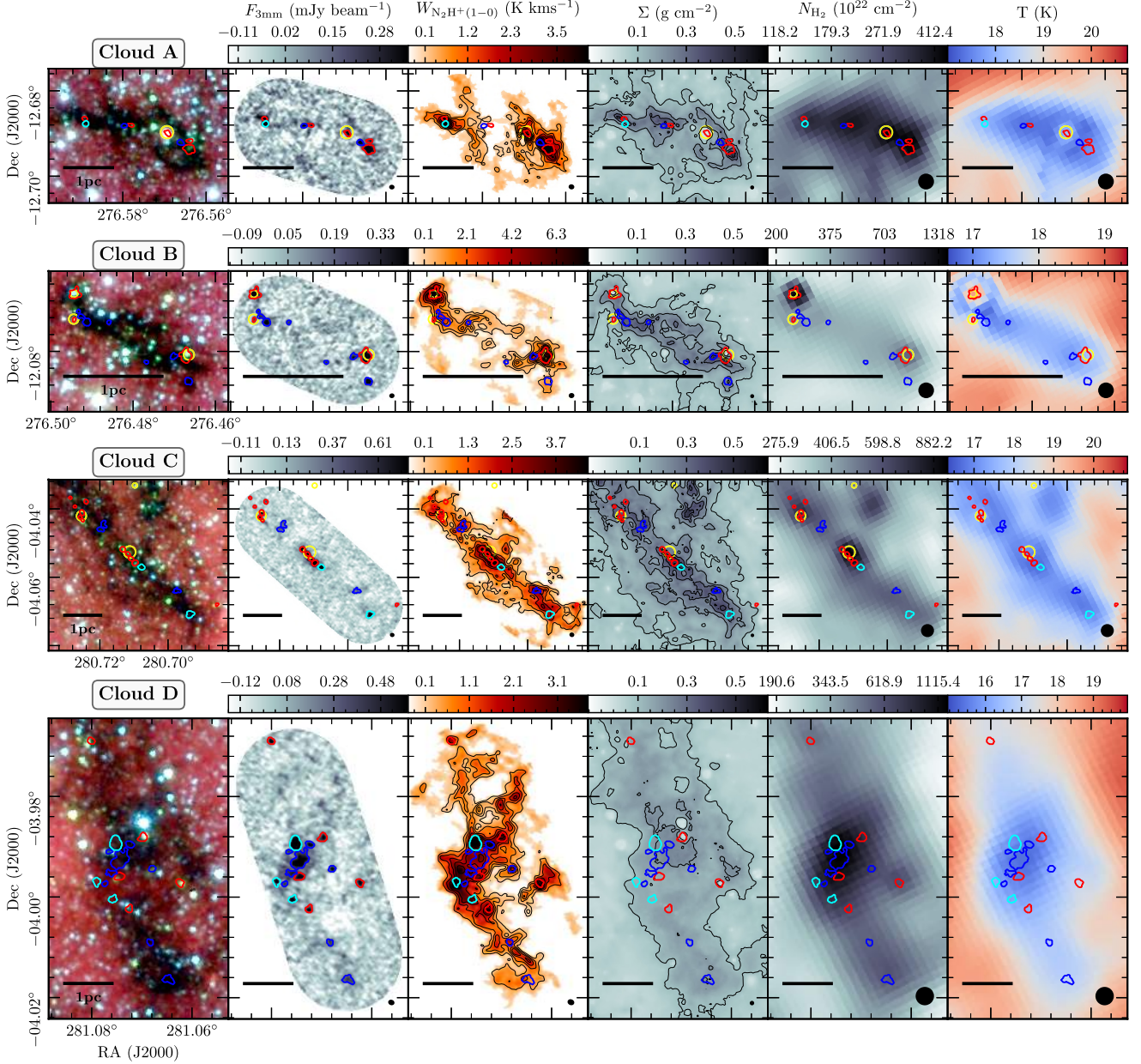
Figure 2. (first column) Three colour images from the Spitzer GLIMPSE survey (Churchwell et al. 2009). (second) The ALMA 3 mm dust continuum (without the primary beam correction), and (third) \text{N}_2\text{H}^+ ( J, F_1, F = 1, 0, 1 \rightarrow 0, 1, 2 ) integrated intensity maps. (fourth) Combined near- and mid-infrared extinction derived mass surface density maps (Kainulainen & Tan 2013). (fifth) Far-infrared Herschel derived column density, and (sixth) dust temperature maps (Marsh et al. 2016, 2017). The yellow circles overlaid on each panel show the positions and sizes of 70\ \mu\text{m} emission point sources (Molinari et al. 2016; Marton et al. 2017). The coloured contours overlaid on each panel show boundaries of all the ‘leaves’ (or cores) identified using the dendrogram analysis on the dust continuum maps (see Section 3.1). The red and blue contours indicate the cores that have been classified as star forming and quiescent, respectively (Section 3.1). The cyan contours indicate the cores that have been identified as being quiescent, high mass, and without further fragmentation (see Section 4.3.2). Shown in the lower left of the ALMA observation panels is the beam size, and in the lower left of the three colour image (first panel) is a scale bar adjusted for the distance of each cloud (see Table 1).
