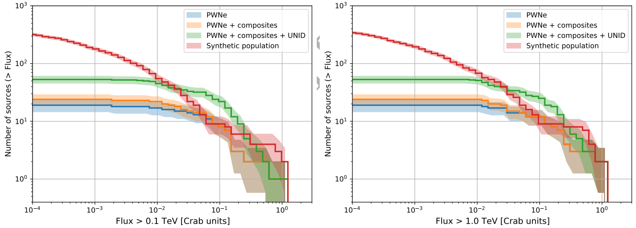
Figure 6. Logarithmic plot of the number of sources emitting in a specific flux range: > 0.1 \text{ TeV} (left panel) and > 1 \text{ TeV} (right panel). The synthetic population (in red) is directly compared with the firmly identified PWNe (in blue), PWNe in a composite SNR (in orange) and the sum of these two with the known unidentified sources (in green). The lighter colored areas represent the errors of each curve.
