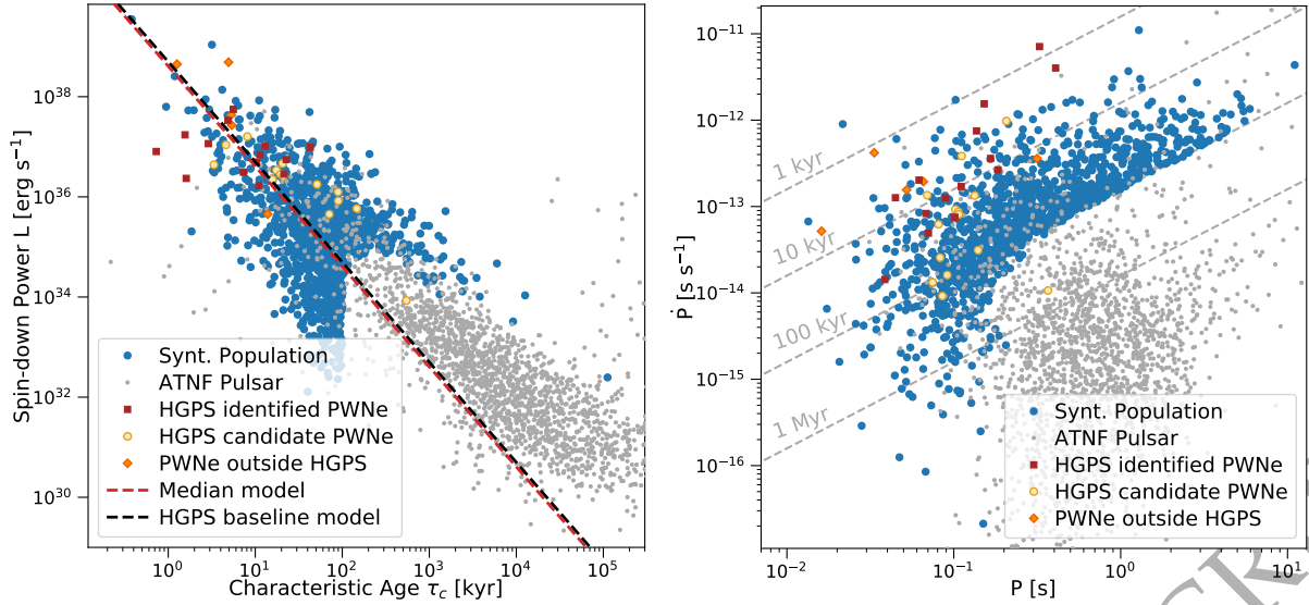
Figure 2. Some characteristic quantities of the chosen population of pulsars (blue circles), to be directly compared with similar plots from Abdalla et al. (2018c) (see e.g. their Fig. 2). The other symbols in the plot represent: PSRs powering PWNe that are firmly identified in the HGPS (red squares); PSRs possibly associated with candidate HGPS PWNe (yellow circles); the 5 PSRs powering nebulae that are included in the HGPS plots as outside HGPS PWNe (orange diamonds), because the associated PWNe are outside the HGPS field, or have not been analysed with the HGPS pipeline (see Abdalla et al. (2018c) for details); all other pulsars from the ATNF catalogue (grey dots). Left Panel: distribution of the pulsars in the characteristic age–luminosity diagram. Dashed lines represent the median of our distribution (red) and the HGPS baseline model (black). Right Panel: distribution of synthetic pulsars in the spin-down period–spin-down period derivative ( P - \dot{P} ) diagram. Dashed lines indicate different characteristic ages of the sources in the population.
