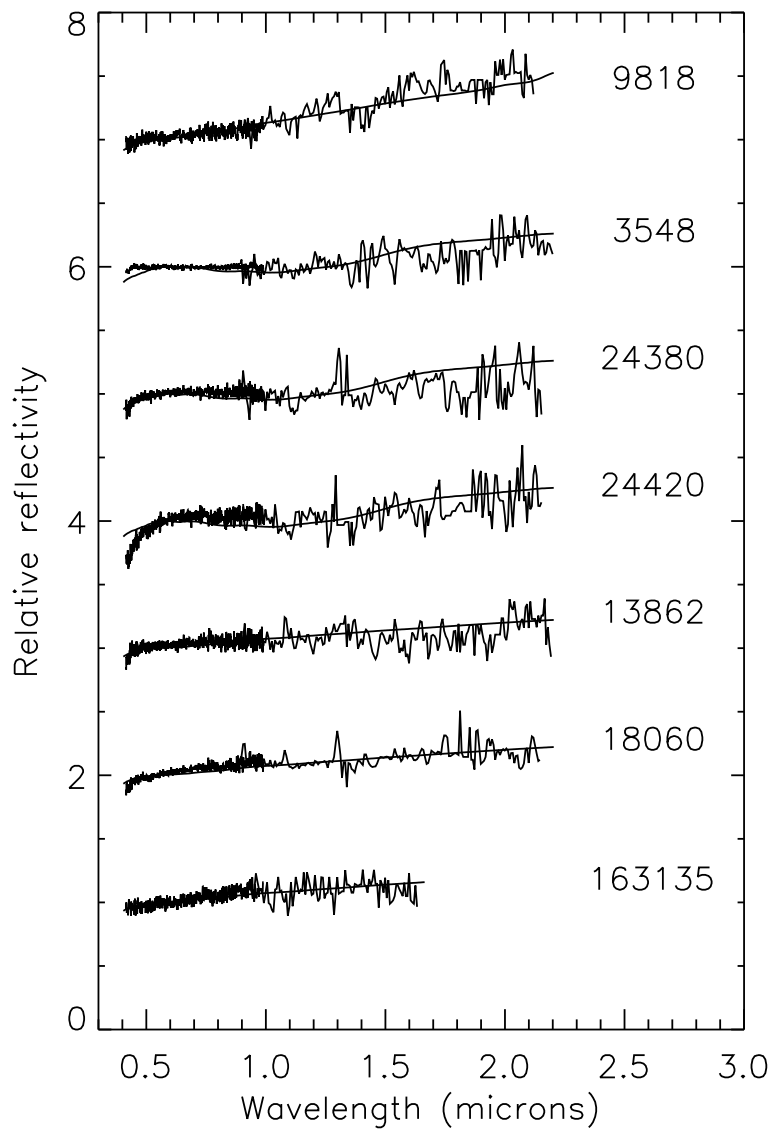
Figure 2: Near-infrared spectra of Eurybates family members obtained by our observations, together with the visible part already published by Fornasier et al. (2007). All the spectra are normalized at 0.55 \mu\text{m} and shifted by 1 in reflectance for clarity. The superimposed continuous lines represent the synthetic spectra obtained modeling the surface composition.
