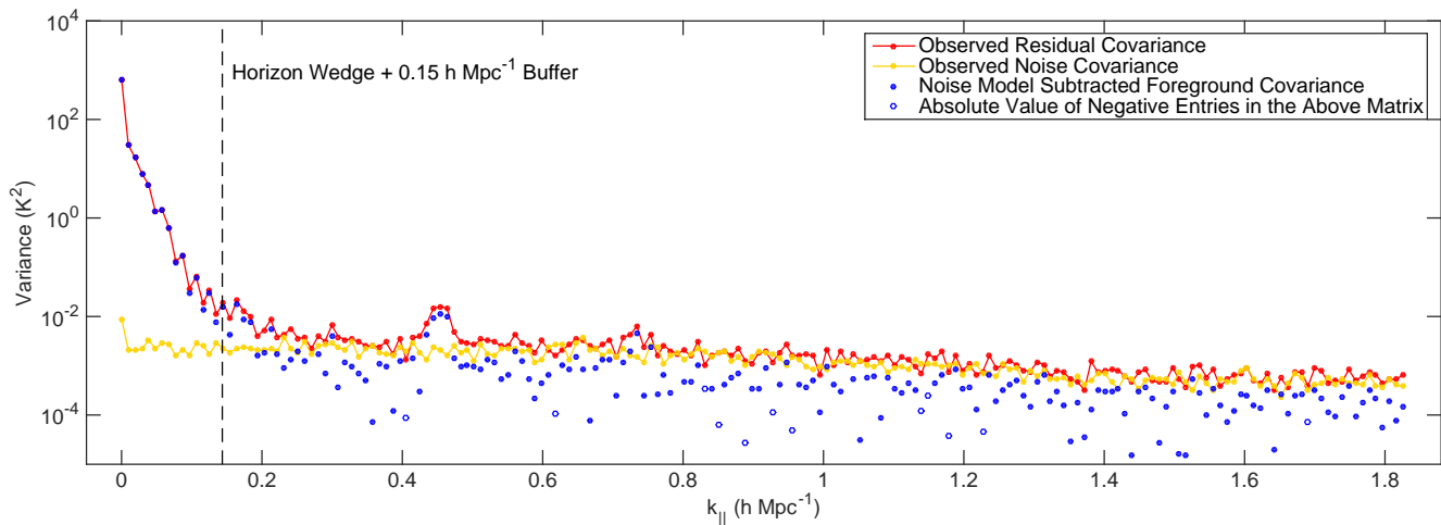
FIG. 2. Examining the diagonal elements of the observed residual and inferred foreground covariance matrices in Fourier space reveals the effectiveness of subtracting model for the noise covariance. In red, we plot the observed residual covariance, which contains both foregrounds and noise. As a function of k_{\parallel} , the two separate relatively cleanly—there is a steeply declining foreground portion on the left followed by a relatively flat noise floor on the right. The theory that the righthand portion is dominated by noise is borne out by the fact that it so closely matches the observed noise covariance, inferred lines of sight of \mathbf{x}_1 - \mathbf{x}_2 , which should have only noise and no sky signal at all. The regions where they differ significantly, for example at k_{\parallel} \sim 0.45 h \text{ Mpc}^{-1} , are attributable to systematic effects like the MWA’s coarse band structure that have not been perfectly calibrated out. For the example covariances shown here (which correspond to a mode in the annulus at k_{\perp} \approx 0.010 h \text{ Mpc}^{-1} ), we can see that subtracting a properly projected noise covariance removes most of the power from the noise-dominated region, leaving only residual noise that appears both as negative power (open blue circle) and as positive power (closed blue circles) at considerably lower magnitude.
