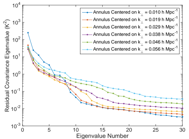
FIG. 1. The evolution of the wedge with k_\perp motivates us to model foregrounds separately for discrete values of k_\perp . In this plot of the thirty largest eigenvalues of the observed residual covariance (which should include both noise and foregrounds) sampled in six concentric annuli, we see steeper declines toward a noise floor for the inner annuli than the outer annuli. This is consistent with the expected effect of the wedge—higher k_\perp modes should be foreground-contaminated at higher k_\parallel .
