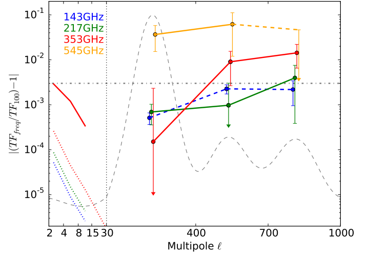
Fig. 41: Transfer function ratio, referred to 100 GHz, for various multipoles. For \ell = 2\text{--}30 , the solid red line is the measured 353-GHz empirical SRoll time TF. The red dotted line shows an upper limit on the 353-GHz residuals after correction, while blue and green dotted lines show an estimate of the residuals at 143 and 217 GHz. The TF for \ell = 30\text{--}1000 is estimated from CMB anisotropies on the first three acoustic peaks (with negative values displayed by dashed lines). The grey dashed line is a CMB power spectrum, showing the position of the first three acoustic peaks.
