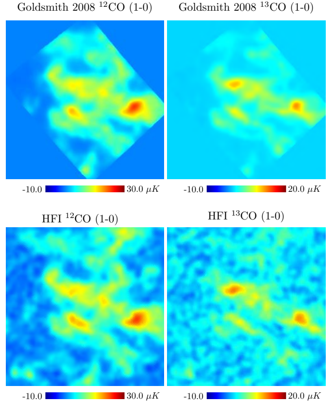
Fig. 6: Top panel : two ground-based radio astronomy maps, centred on (173^\circ 0', -16^\circ 0') in Galactic coordinates, at ^{12}\text{CO} and ^{13}\text{CO} in the Taurus region. Bottom panel : HFI ^{12}\text{CO} and ^{13}\text{CO} maps extracted by SRo11.
