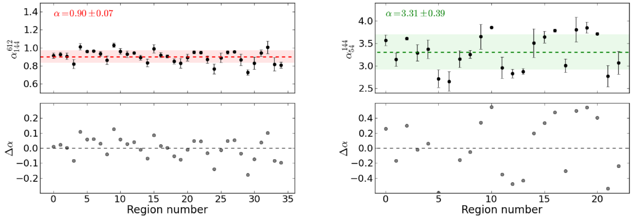
Figure 9. Spectral index distribution across the mini halo (left-hand panel, \alpha_{612}^{144} ) and across the SW diffuse emission (Right-hand panel, \alpha_{54}^{144} ). The spectral indices were extracted in regions indicated in Fig. 6 (red squares) and in Fig. 7 (green square), respectively. The dashed horizontal line indicates the mean spectral index, while the coloured region represents the standard deviation. The lower panels show the residuals of \alpha with respect to the mean spectral index.
