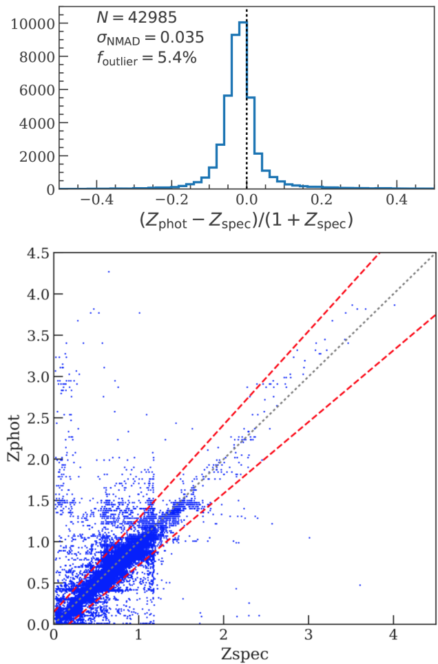
Figure C1. Spectroscopic and photometric redshifts for the 42985 sources with high-quality photo- z s and spec- z s in the 4.5 deg 2 region covered by the N18 forced-photometry catalogue (sources identified as a broad-line AGN were excluded, see Section 5.1). The top panel shows the histogram of the fractional difference between the spec- z s and the photo- z s. The bottom panel shows the direct comparison between the spec- z s and the photo- z s. The black dotted lines in both panels mark the z_{\text{spec}} = z_{\text{phot}} relation. In the bottom panel, the red dashed lines mark the |\Delta z|/(1 + z_{\text{spec}}) = 0.15 thresholds for outliers.
