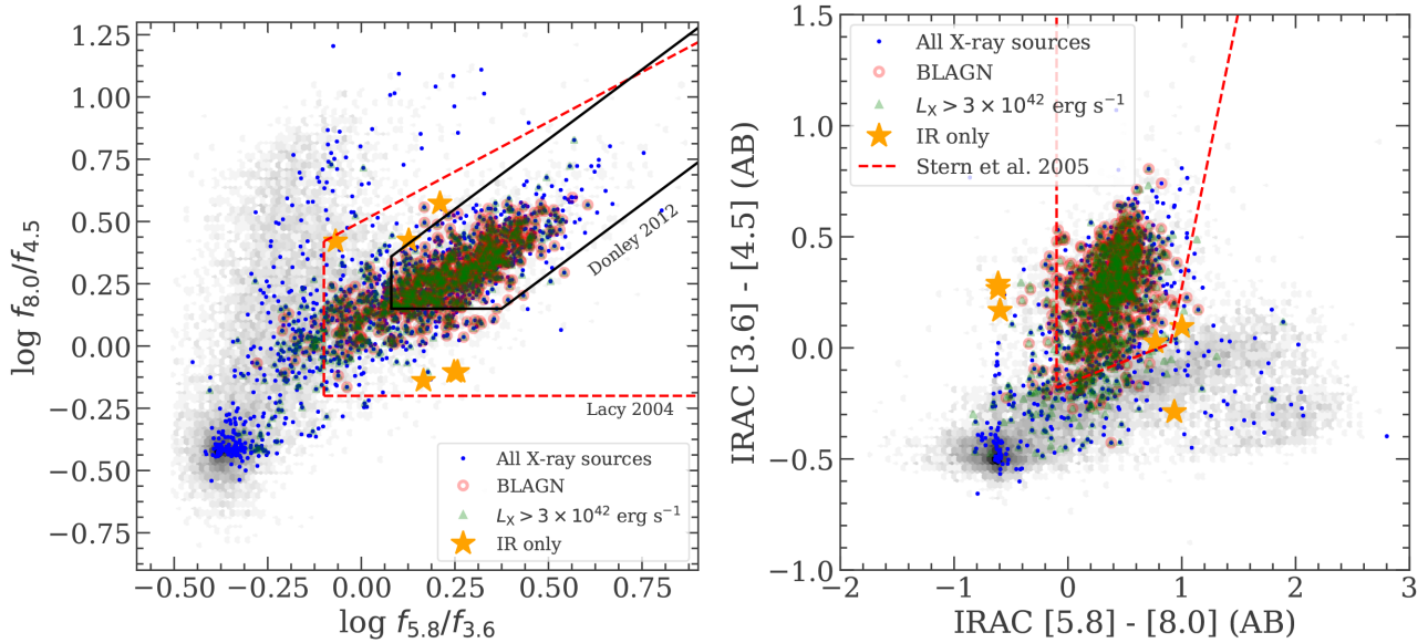
Figure 24. Left: \log f_{5.8}/f_{3.6} versus \log f_{8.0}/f_{4.5} distribution. Right: IRAC[5.8] – [8.0] versus [3.6] – [4.5] (AB) distributions. In both panels, the Spitzer IRAC two-colour distribution for the 1716 X-ray sources with detections in all four IRAC bands are shown as the blue dots. X-ray luminous AGNs and spectroscopically confirmed quasars are also shown as the green triangles and the open red circles, respectively. There are a total of 1325 sources with IRAC colours satisfying one of the three mid-IR colour AGN selection criteria (Lacy et al. 2004; Stern et al. 2005; Donley et al. 2012). The six sources that are only identified as an AGN based on their IRAC colours are displayed as the large orange stars. The colour distribution for the 12990 SWIRE sources in our X-ray catalogue region is also shown as the grey hexagonal cells, where darker colour indicates higher source density.
