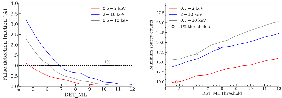
Figure 6. Left: The fraction of spurious sources detected at different \text{DET\_ML} based on simulations. The detection threshold relevant to our catalogue is marked as the horizontal dashed line. Right: The minimum source counts for the detected sources (the median of all 20 simulations) with \text{DET\_ML} values above a given \text{DET\_ML} threshold. As expected, higher \text{DET\_ML} thresholds can only detect sources with higher numbers of counts. The \text{DET\_ML} values corresponding to the 1 per cent spurious fraction are marked as the open circles.
