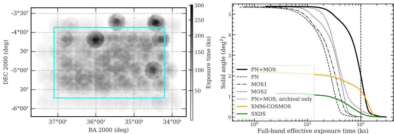
Figure 3. Left: Full-band survey effective exposure map (PN + MOS). The 5.3 \text{ deg}^2 survey region from which the X-ray source catalogue is constructed is marked as the cyan rectangular box. Except for several regions with deep XMM–Newton follow-up observations of galaxy clusters, the XMM–Newton coverage in our survey region is generally uniform. Right: The black solid line shows the cumulative survey solid angle as a function of full-band effective (i.e. vignettted) PN+MOS exposure for observations used in this work. Distributions for individual instruments are indicated as the dashed line (PN), dash-dotted line (MOS1), and dotted line (MOS2). For comparison, the cumulative survey solid angle for the archival XMM–Newton data in our survey region, in XMM-COSMOS, and in SXDS are shown as the thin purple line, thick orange line, and thick green line, respectively. The dashed vertical line marks exposure time = 100 ks.
