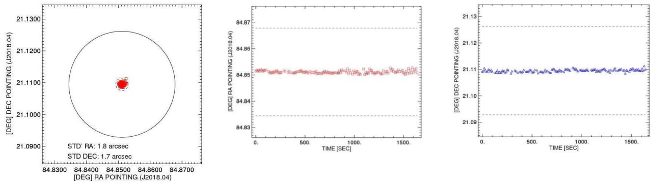
Figure 4. Pointing and tracking performance of the ASTRI telescope. Left: RA-DEC plot showing that the position of the telescope can be measured with an accuracy within the 7 arcsec (dashed circle) requested by the CTA requirement of post calibration astrometric accuracy. Center and right: RA and DEC plots versus time showing that ASTRI is well within the 1 arcmin (dashed lines) online astrometric accuracy requested by CTA.
