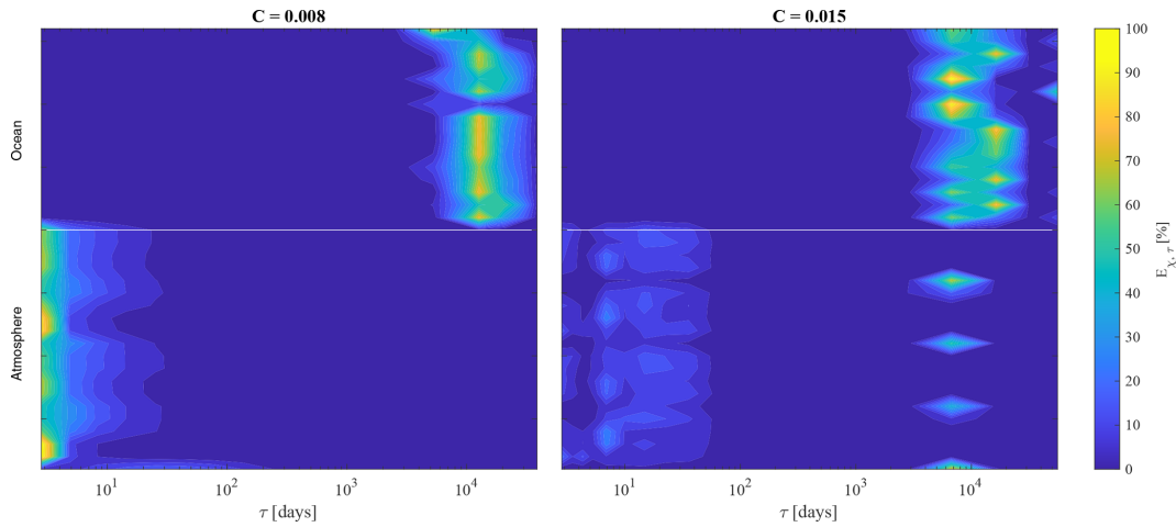
Figure 3. Relative contribution (in percentage) E_{\chi,\tau} of each variable \chi = \{\psi_{a,i}, \theta_{a,i}, \Psi_{o,i}, T_{o,i}\} in dependence on the mean timescale \tau . Panels (a) and (b) refer to the two values of the friction coefficient C = 0.008 and C = 0.015 , respectively. The white line separates the atmospheric variables from the oceanic ones.
