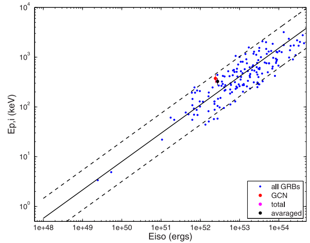
Figure 2. Our GRB compared to the whole sample of GRBs until 2013 June. The solid line is E_{p,i} = 110 * E_{\text{iso}}^{0.57} , while the dashed line is the 2\sigma standard deviation (Amati et al. 2009).
