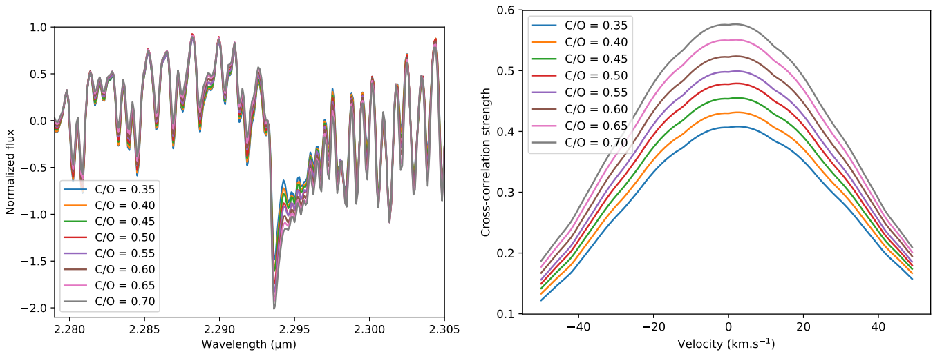
Fig. C.2. Investigations of the characterization performances using the molecular mapping. Left: zoom into the \nu = 2-0 CO overtone at 2.29 \text{ }\mu\text{m} of normalized continuum-subtracted Exo-REM models at different C/O ratios ( T_{\text{eff}} = 1650 K, \log(g) = 4.0 dex, [M/H] = 0.0 and C/O = 0.35–0.70). Right: CCF between the Exo-REM models and the CO template shown in Fig. 4.
