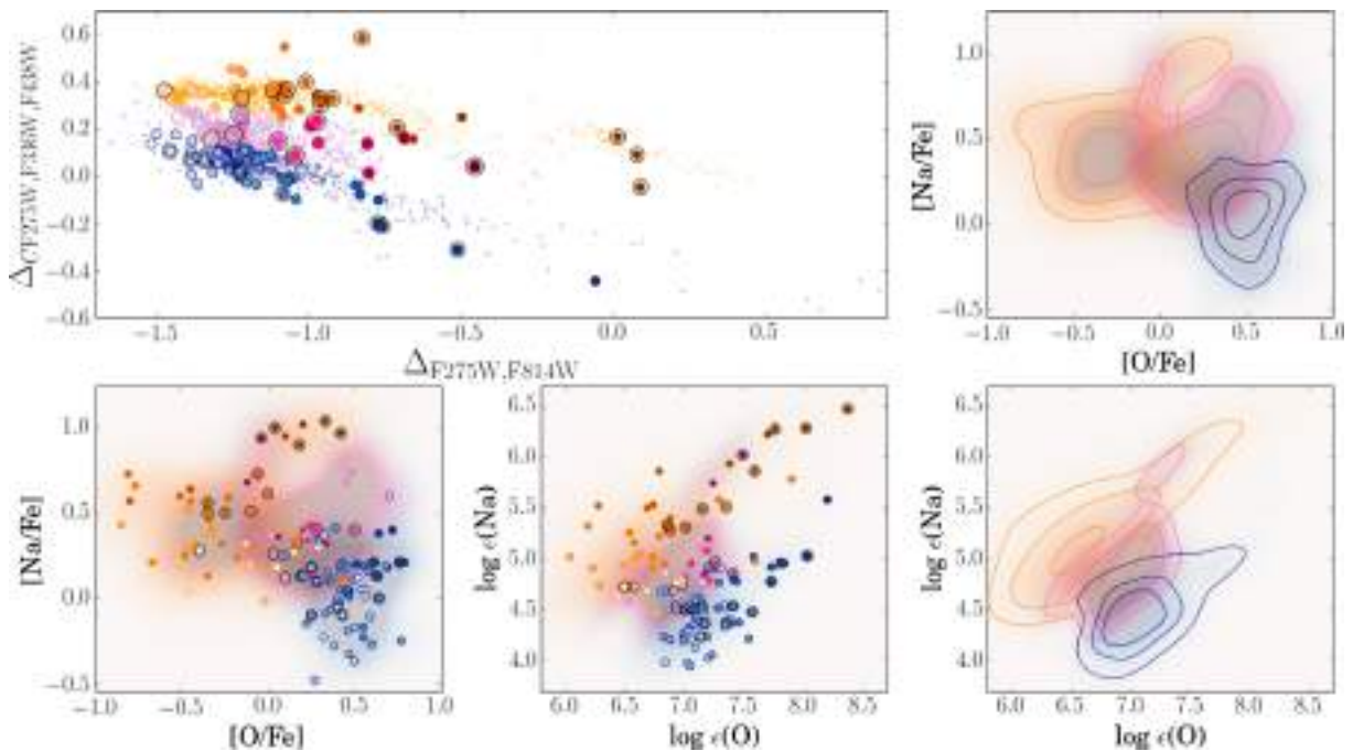
Figure 23. Chromosome map of \omega Centauri (top-left panel): three main streams of stars are evident at different levels of \Delta_{C F275W, F336W, F438W} . The lower, middle, and upper streams have been coloured in light blue, pink and orange colours, respectively. Larger dots are stars with available chemical abundances from spectroscopy from Johnson & Pilachowski (2010, dots without the black circles) and Marino et al. (2011b, black-circled points). Oxygen abundances from Johnson & Pilachowski (2010) have been shifted by +0.15 dex to account for the systematic difference with the O abundances inferred by Marino et al. (2011b). To each star with spectroscopic data a gradient in colour has been assigned proportional to its \Delta_{F275W, F814W} value. In the lower-left and -middle panels we represent the observed Na-O anticorrelation in abundances relative to Fe (left) and in absolute abundances (middle) for the stars represented on the ChM. The two right-side panels represent the same Na-O planes with contour density levels for stars belonging to each separate stream of the map.
