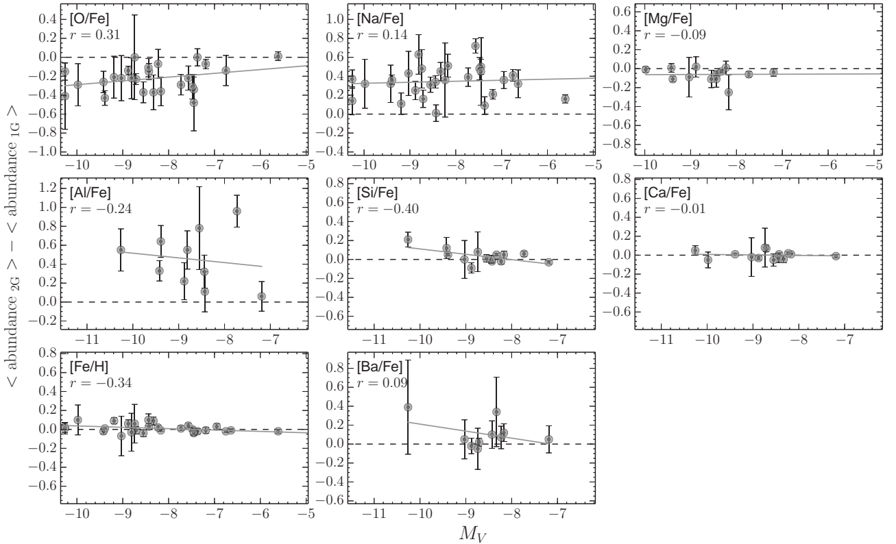
Figure 19. Abundance differences relative to Fe ( \langle \text{abundance}_{2\text{G}} \rangle - \langle \text{abundance}_{1\text{G}} \rangle ) (and relative to H in the case of Fe) between 2G and 1G stars (from Table 2) as a function of the absolute magnitude M_V . Error bars are the square root sum of the statistical errors associated with the average values ( \text{rms}/\sqrt{N-1} ), with N the number of measurements) of 1G and 2G stars; when only one measurement is available, the statistical error has been assumed equal to 0.20 dex. The dashed black line indicates no difference. For comparison purposes, the x - and y -axes have the same size in all the panels. Each panel reports the Spearman correlation coefficient r .
