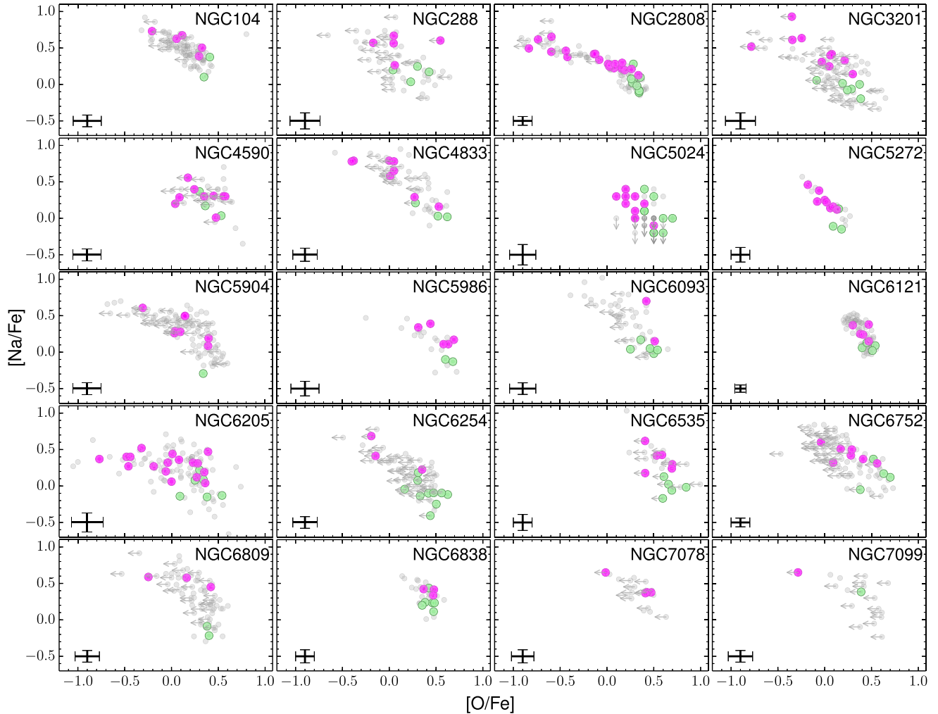
Figure 8. [\text{Na}/\text{Fe}] versus [\text{O}/\text{Fe}] for 20 Type I clusters for which both sodium and oxygen abundances are available from the literature. 1G and 2G stars are represented with large green and magenta dots, respectively. The entire sample with spectroscopic abundances is represented with grey dots. The typical error bars are taken from the reference papers listed in Table 1.
