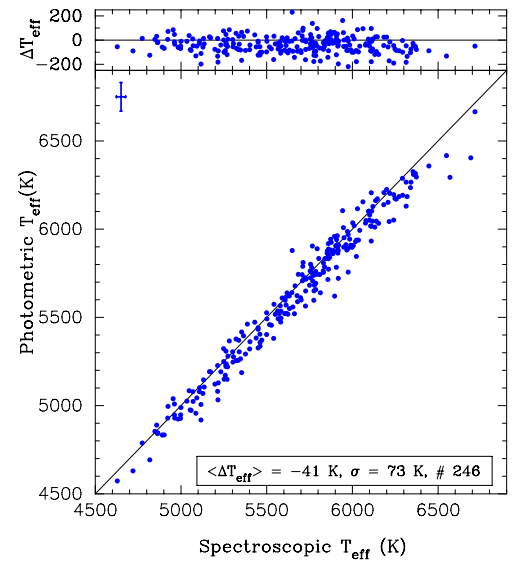
Fig. 1. Comparison between our spectroscopically derived T_{\text{eff}} and those obtained from (B - V) colours. The upper panel shows the differences between the photometric and the spectroscopic values. Mean uncertainties in the derived temperatures are also shown.
