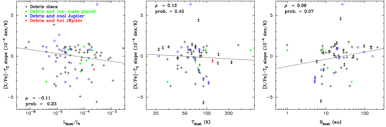
Fig. 13. T_C^{\text{all}} -slope as a function of the dust parameters, fractional dust luminosity L_{\text{dust}}/L_* (left panel), dust temperature T_{\text{dust}} (middle panel), and disc radius R_{\text{disc}} . A linear fit to the data is shown by the grey continuous line. Results from the Spearman's correlation test are also shown in the plot (lower/upper limits are not considered in the statistics).
