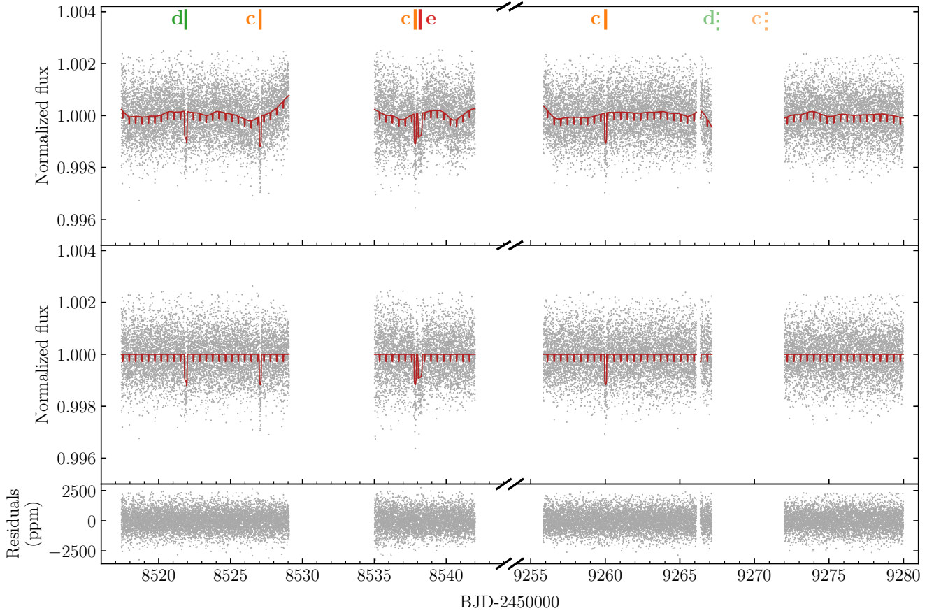
Figure 1. TESS sector 8 ( left ) and 35 ( right ) PDCSAP light curves of TOI-561. In the top panel, the dark red solid line shows the best-fitting transit and Matérn-3/2 kernel Gaussian Process (GP) model, as detailed in Section 5. The central panel shows the flattened light curve after the removal of the GP component, with the best-fitting transit model superimposed (dark red solid line). The transits of planets c, d and e are labelled and highlighted with orange, green and red vertical lines, respectively. The expected locations of the transits of planets c and d occurring during the data gaps of sector 35 are marked with pale, dashed orange and green lines, respectively. Planet e is not expected to transit in sector 35. The transits of the USP planet are too shallow to be individually visible, and are not indicated. Light curve residuals are shown in the bottom panel.
