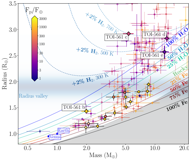
Figure 11. Mass-radius diagram for exoplanets with radii and masses measured with a precision better than 30%, colour coded according to their incidental flux. Data are taken from the Extrasolar Planets Encyclopaedia catalogue ( http://exoplanet.eu/catalog/ ) as of 18 October 2021. The TOI-561 planets are labelled, and highlighted with coloured diamonds. The USP planets are emphasized with thick, black-contoured circles. The theoretical mass-radius curves for various chemical compositions (Zeng et al. 2019) are represented by solid coloured lines, while the dashed lines indicate the curves for an Earth-like core surrounded by a H 2 envelope (2% mass fraction) at varying equilibrium temperatures. The forbidden region predicted by collisional stripping (Marcus et al. 2010) is marked by the shaded grey region.
