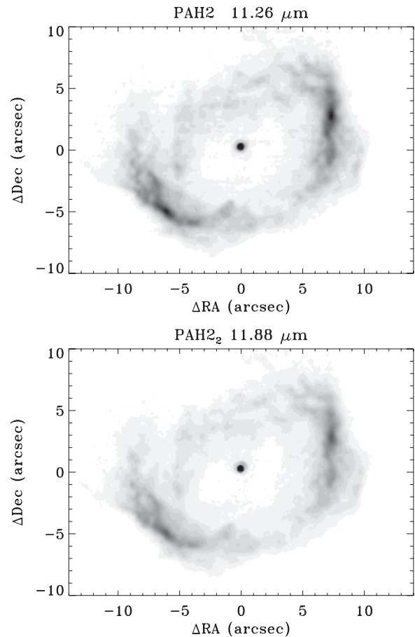
Figure 5. VISIR maps of HD 168625 on the 11.2 \mu\text{m} PAH feature (upper panel) and the adjacent continuum (lower panel). In both panels, the brightness levels range from 0 to 2.48 \text{Jy arcsec}^{-2} . The central star has a peak of 10.95 and 10.58 \text{Jy arcsec}^{-2} in the two maps. The brightest point in the nebula is 2.41 \text{Jy arcsec}^{-2} and 1.82 \text{Jy arcsec}^{-2} , respectively.
